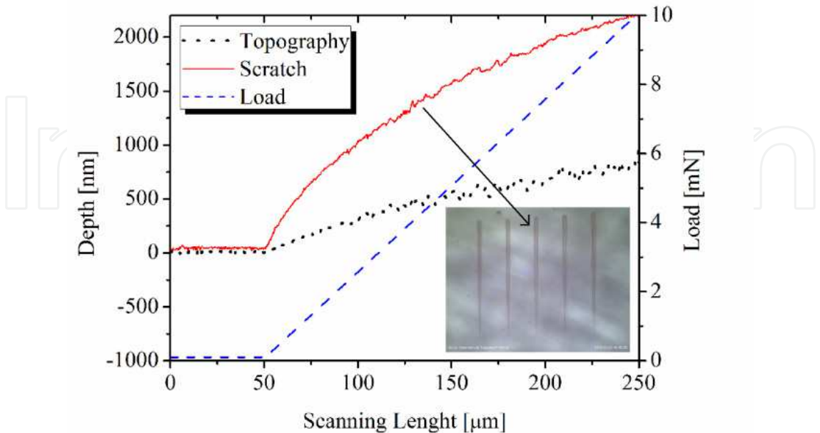
Fig. 8. Scratch test curve of SiO 2 layer of treated AryLite™ with optical image in the plot inset (magnification 20x). Topography and scratch scan refers to the third wear
