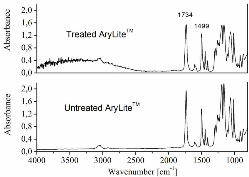
Fig. 4. ATR spectra of AryLite™ before and after surface silane treatment in the range 4000-700 cm -1
