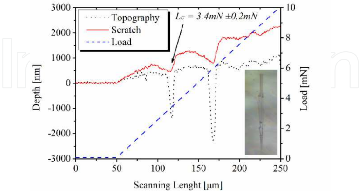
Fig. 7. Scratch test curve of SiO 2 layer of untreated AryLite™ with optical image in the plot inset (magnification 20x)
