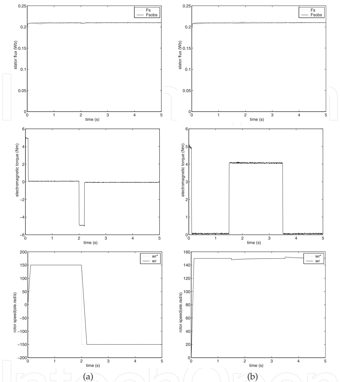
Fig. 5. Simulation results from neural observer: (a) speed reversal with no load in t=2s ; (b) loading and unloading (constant torque) the motor at constant speed of 150 ele.rad/s in t=1.5s and t=3.5s , respectively.
