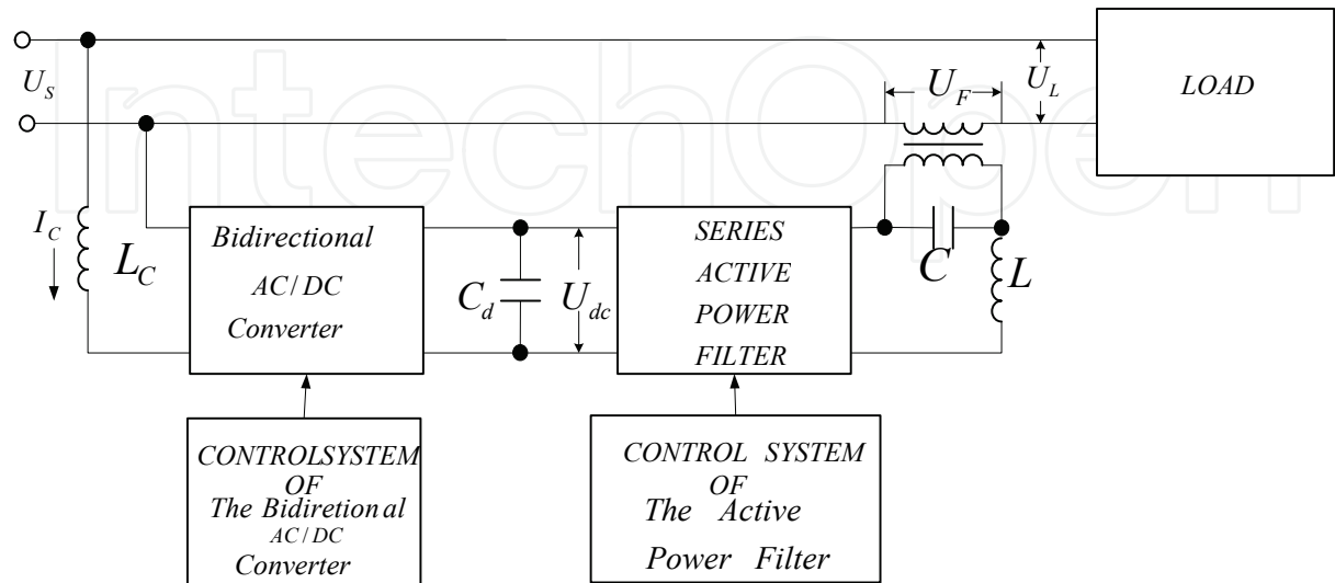
Fig. 18. Block diagram of a precise stabilizer-filter of AC voltage
