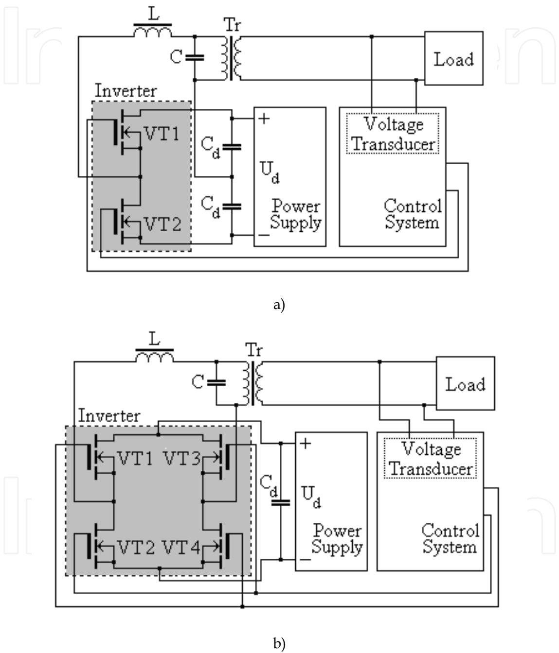
Fig. 1. a) half-bridge and b) bridge circuits of an inverter
