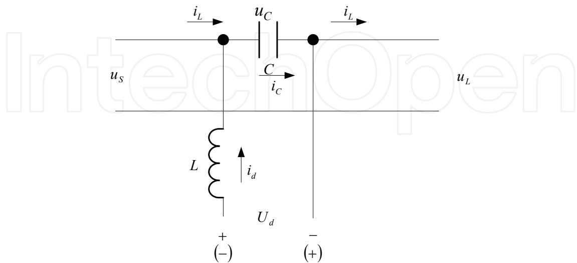
Fig. 15. Circuit used to make the analysis of sliding mode control of the series active power filter
