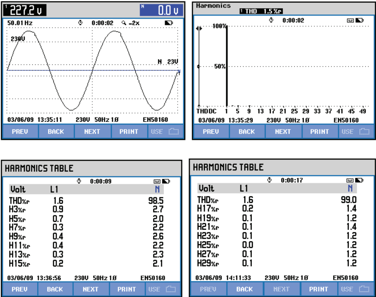
Fig. 21. Parameters of the load voltage when stabilizer – APF is switched on Fig.24 shows transient processes at a sharp change of the source voltage. The reason that the sinusoidal waveform of the voltage is not seen is that the scale of the X-axis is 1s/div. The aim of this presentation is to be more clear that the value of the voltage feeding the load do not change significantly at a sharp change of the source voltage (both when its value decreases or increases) when the precise stabilizer-filter is switched on.
