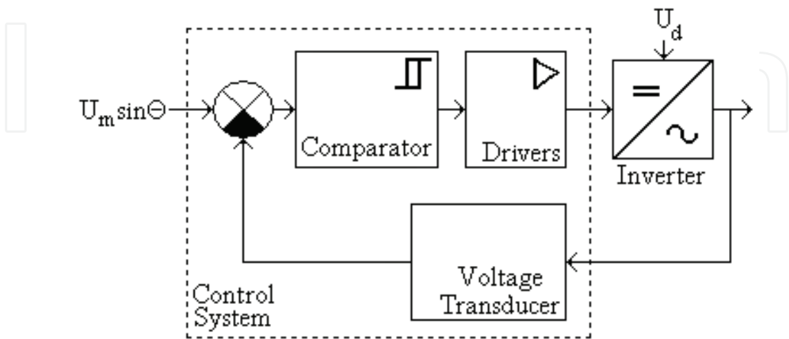
Fig. 2. Block diagram of the control system with hysteresis control
