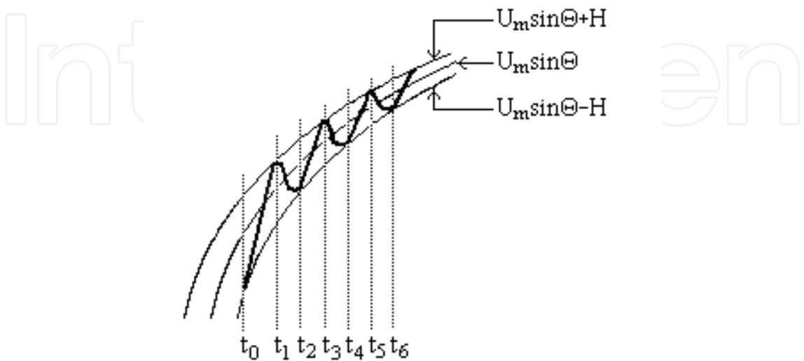
Fig. 3. Explanation of the sliding- mode control
