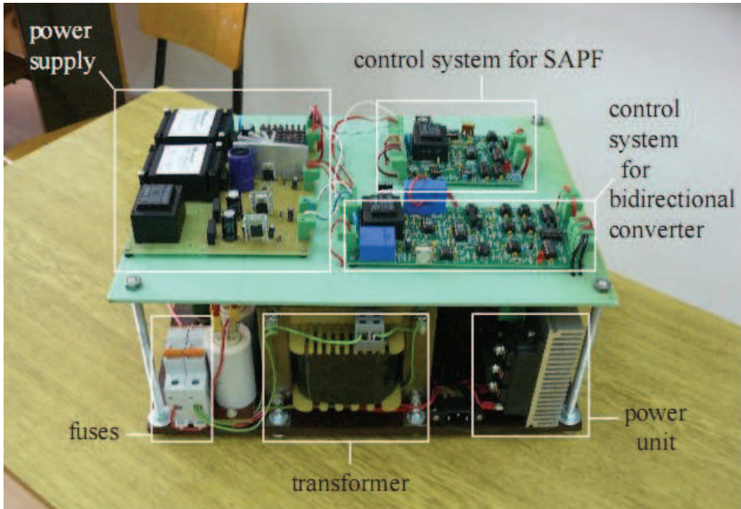
Fig. 19. Single-phase precise stabilizer-filter of AC voltage
