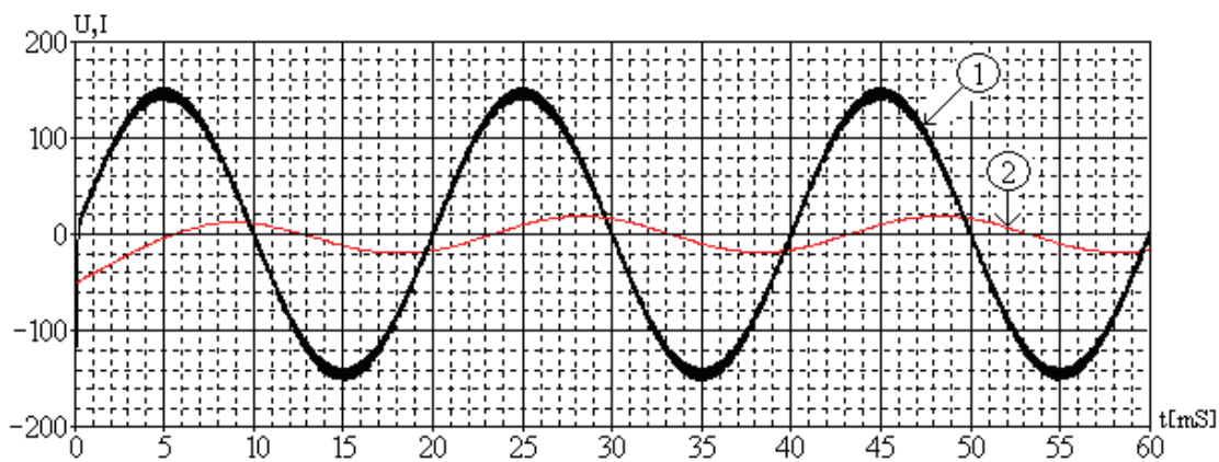
Fig. 8. Computer simulation results of the inverter operation with an active-inductive load equal to 400\Omega/2\text{H} using sliding mode control. Curve 1 – the voltage feeding the load, curve 2 – the load current
