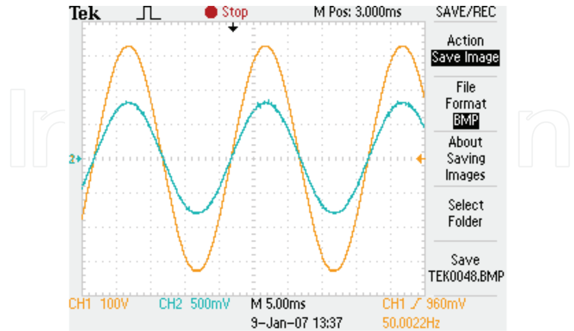
Fig. 10. The load voltage and load current in the case of active load
