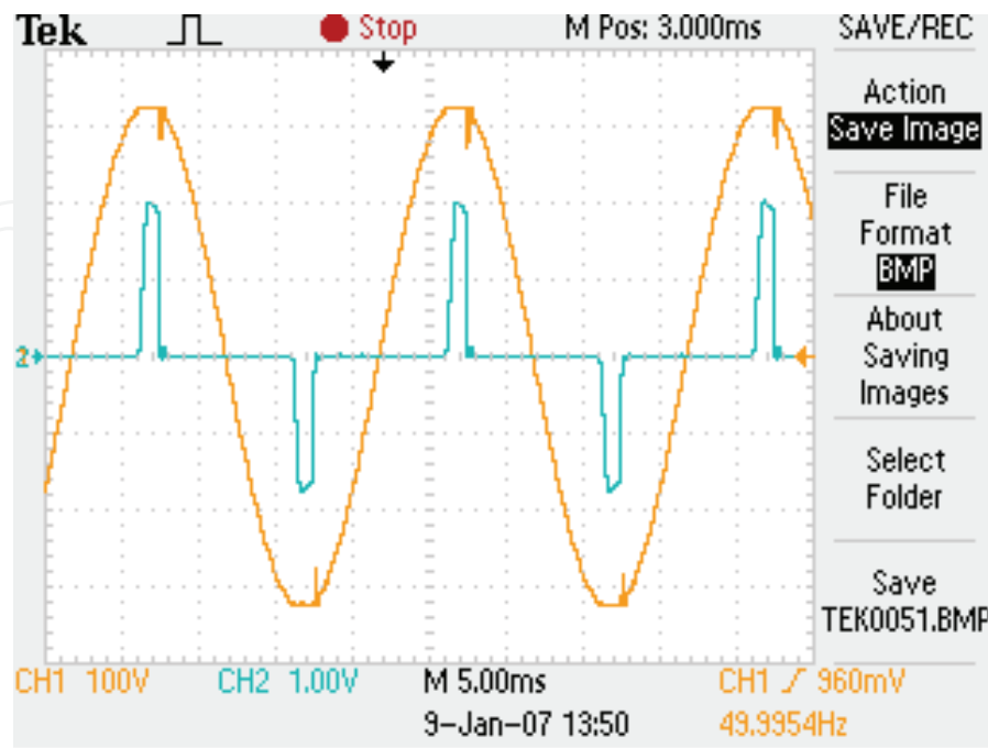
Fig. 13. The load voltage and load current in the case of single-phase bridge rectifier
