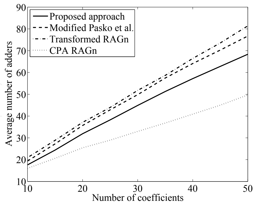
Fig. 15. Average number of adders for sets with 12-bits coefficients.
