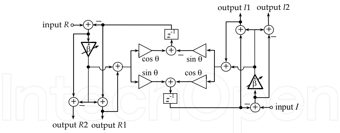
Fig. 13. Variable complex LS1b digital filter structure.
