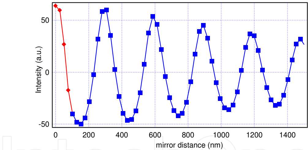
Fig. 14. Corrected interferogram to obtain the spectrum in Fig 12 and Fig 13. Blue squares: the original incomplete interferogram, red diamonds the reconstructed four points
