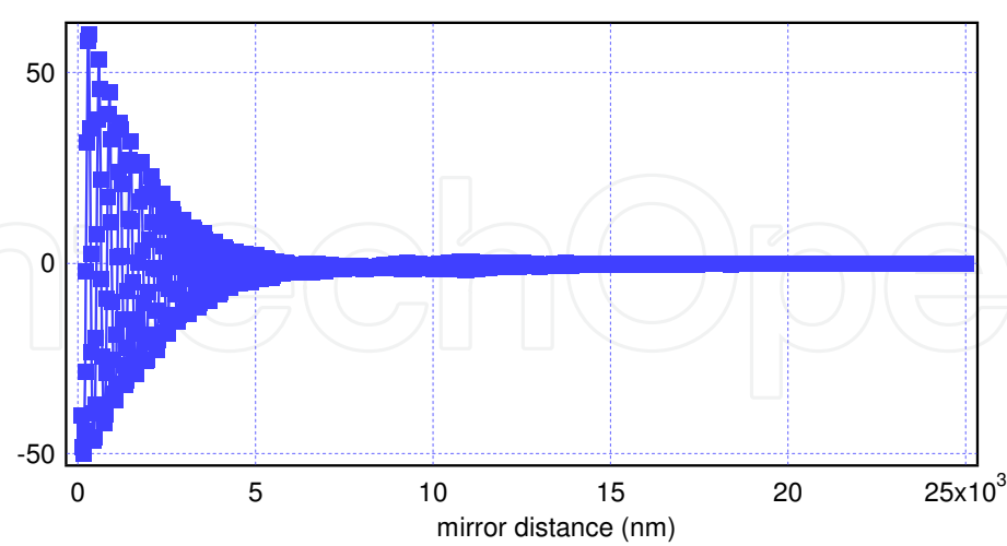
Fig. 9(a). The interferogram of a yellow LED with a maximum mirror distance \delta = 25\text{ }\mu\text{m} The two aforementioned problems (presence of harmonics and missing points) are solved in our prototype by introducing an optical bandpass filter in the optical system transmitting slightly less than one octave of the electromagnetic spectrum, as the spectrum reported in Fig 7(b). This solution reduces the region of measurable spectrum but has the important
