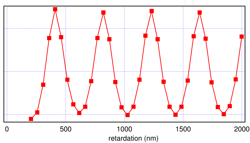
Fig. 8. The measured interferogram of a laser radiation at \lambda = 410\text{ nm} . The estimated penetration depth of the metallic layer is smaller than 50 nm
