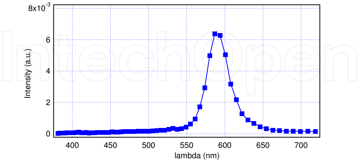
Fig. 13. The spectrum versus wavelength of the yellow LED in Fig 12
