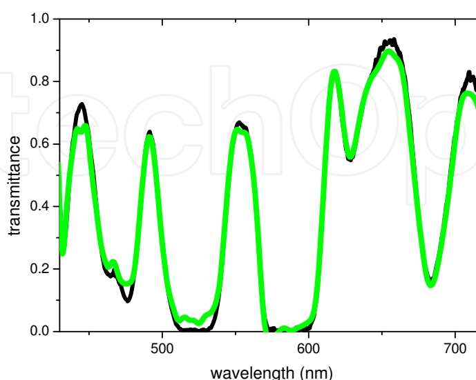
Fig. 22. The complex transmission spectrum of a glass doped with didymium oxide. The black line is the same spectrum measured with a classical spectrometer
