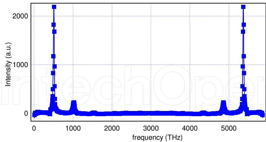
Fig. 12. The spectrum versus frequency of the yellow LED obtained by reconstructing the four missing points
