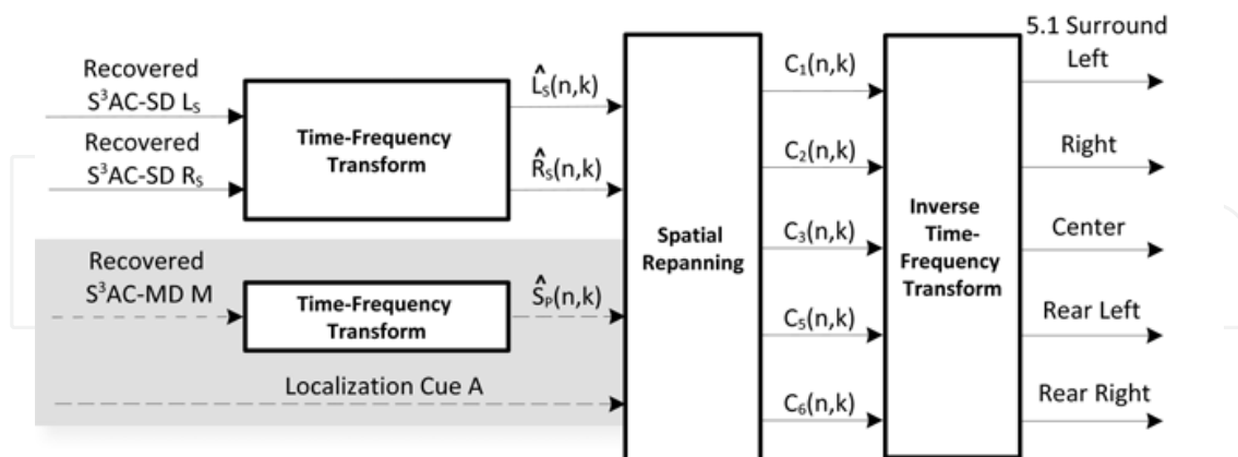
Fig. 4. S 3 AC Decoder illustrating the processing of time domain signals recovered by the AMR-WB+ decoder to produce time-domain loudspeaker signals for reproduction of the spatial teleconference audio at each site.
