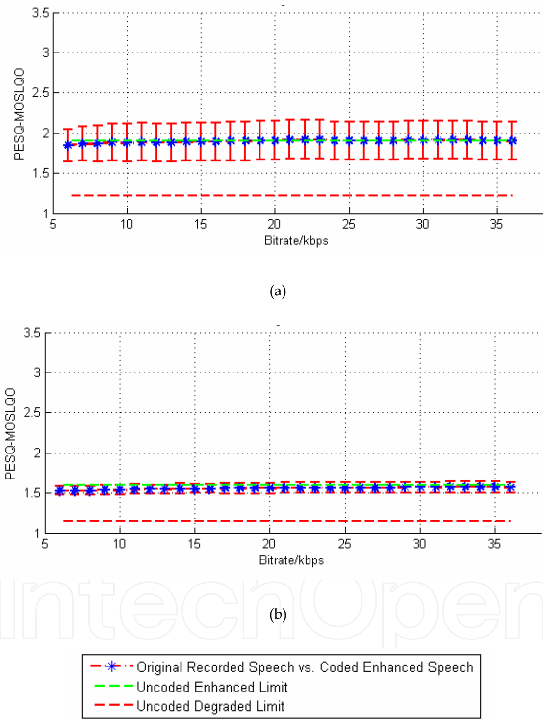
Fig. 11. Average results for recordings in diffuse noise across all noise sources for an SNR of 0 dB (a) Anechoic recordings. (b) Echoic recordings. Blue asterisk curves: results for PESQ of the decoded outputs from AMR-WB+ compared with the original clean speech. Green dashed curves: results when no AMR-WB+ coding is applied to the enhanced recordings. Red dashed curves: results obtained when coding the non-enhanced recordings.
