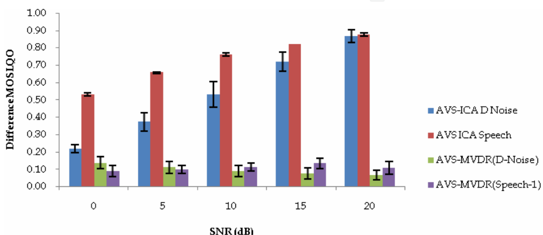
Fig. 9. Difference MOS Vs SNR in reverberant conditions.
