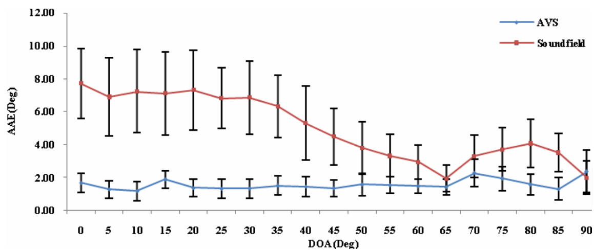
Fig. 7. Average Angular Error (AAE) for theDOA estimated for for recordings of speech from teh AVS and the SoundField microphones. Reocrdngs were made in reverberant conditions.
