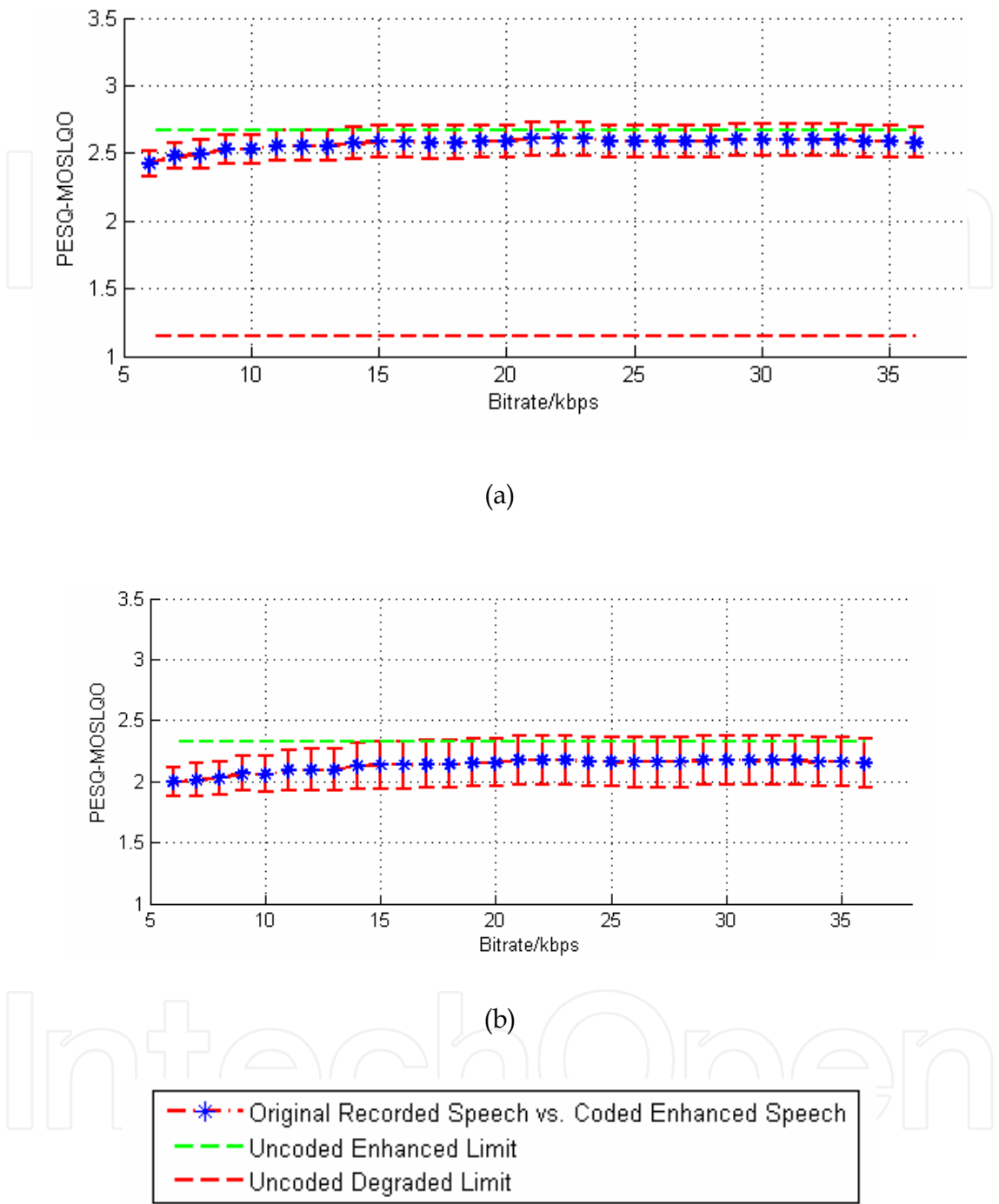
Fig. 12. Average results for recordings in diffuse noise across all noise sources for an SNR of 20 dB. (a) Anechoic recordings. (b) Echoic recordings. Blue asterisk curves: results for PESQ of the decoded outputs from AMR-WB+ compared with the original clean speech. Green dashed curves: results when no AMR-WB+ coding is applied to the enhanced recordings. Red dashed curves: results obtained when coding the non-enhanced recordings.
