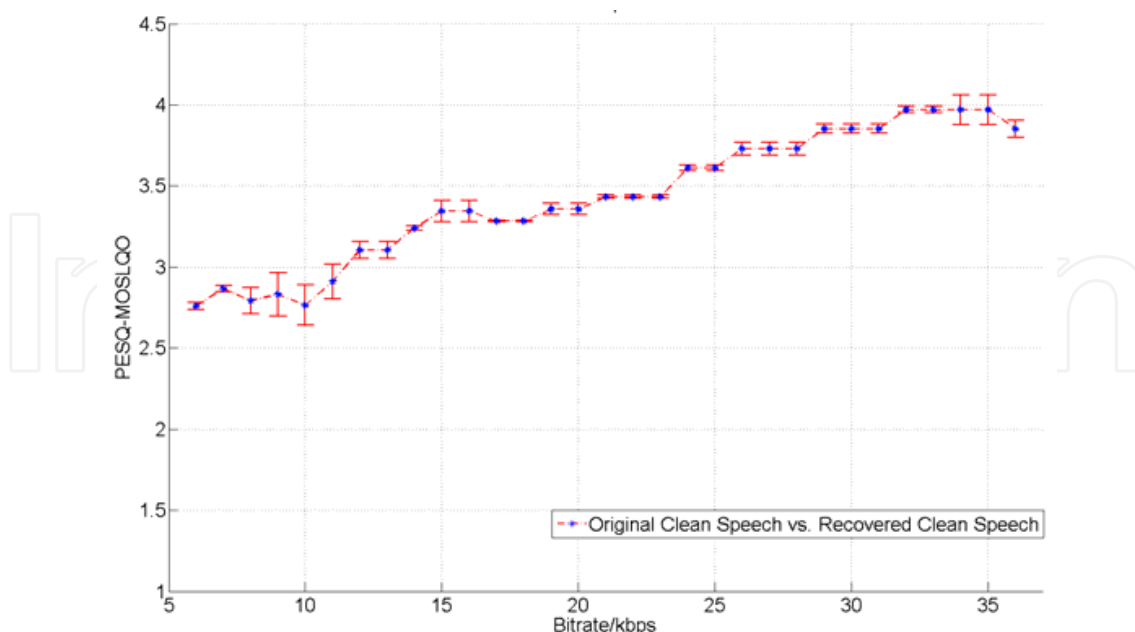
Fig. 10. PESQ results for original clean speech coded using the proposed spatial teleconferencing system including downmix compression via AMR-WB+.
