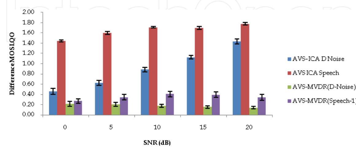
Fig. 8. Difference MOS Vs SNR in Anechoic Conditions
