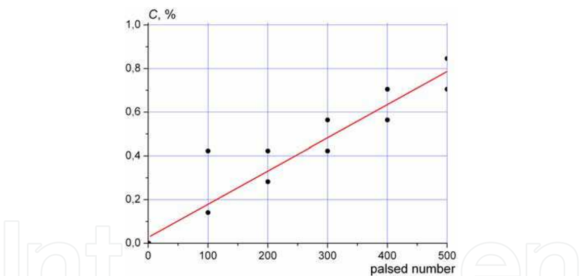
Fig. 17. The dependence of the conversion level of methane pyrolysis on the number of pulses in the electron beam.
