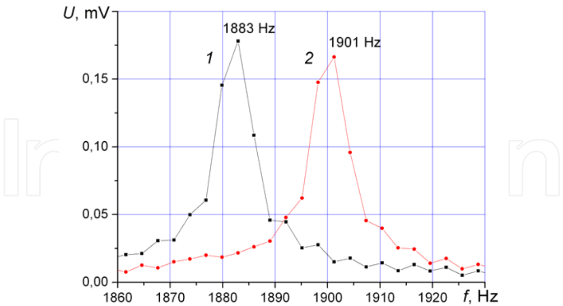
Fig. 16. The spectrum of sound waves in methane: initially (1), and after irradiation by 500 pulses: (2).
