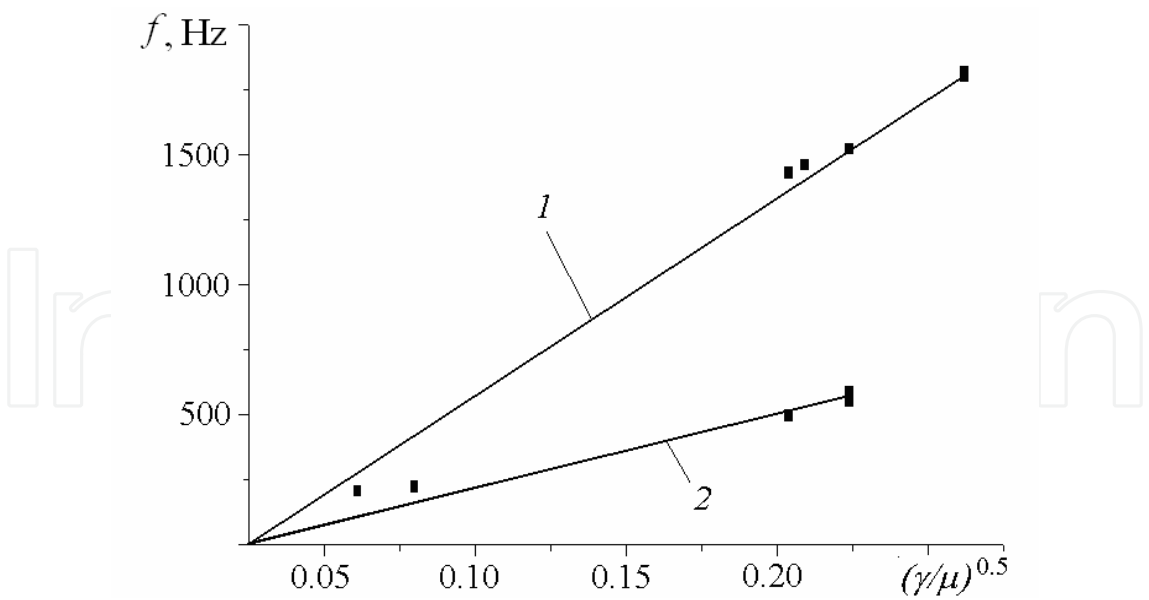
Fig. 8. The dependence of the frequency of the sound vibrations in the reactor on the ratio of the adiabatic exponent to the molar mass of single-component gases. Dots correspond to experimental data, lines are the calculations by (Eq.1) at l = 11.5 cm (1) and 30 cm (2).
