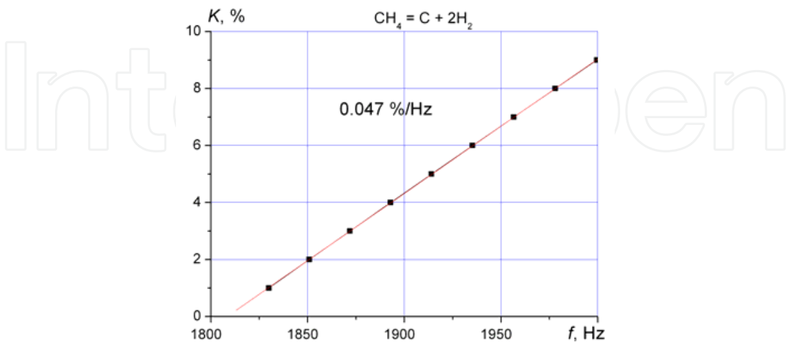
Fig. 14. Dependence of the conversion level of methane in the pyrolysis reaction on the frequency of transverse sound waves.
