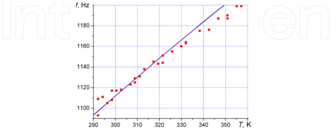
Fig. 10. The dependence of the frequency of transverse sound waves on the gas temperature. The points correspond to the experimental values, the lines - calculation by (2).
