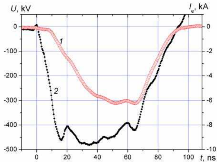
Fig. 3. Oscilloscope traces of electron current (1) and accelerating voltage (2) These graphs are averaged for 10 pulses with a frequency of 1 impulse/s after operating the cathode for 10–20 pulses. The parameters of the electron beam are given in Table 1.
