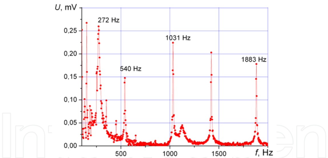
Fig. 15. The spectrum of sound waves in a reactor filled with methane after injection of high-current electron beam.
