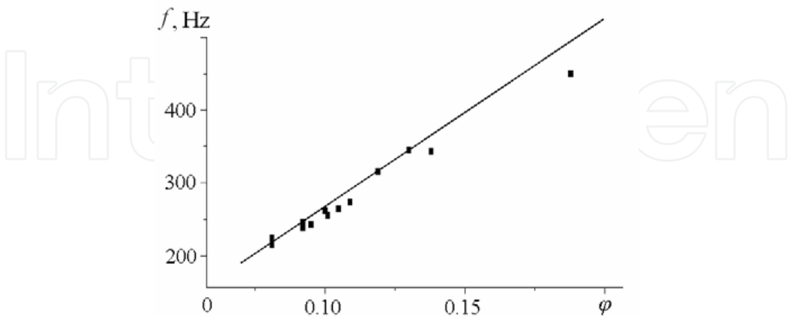
Fig. 9. The dependence of the frequency of sound oscillations in the plasma chemical reactor with a length of 30 cm on the parameter \varphi for gas mixtures. The points correspond to the experimental values, the lines are calculated from (3).
