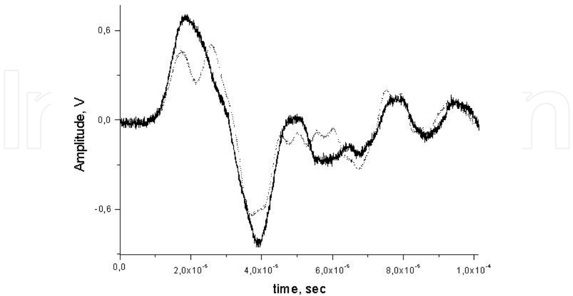
Fig. 23. Oscilloscope traces for different profiles of the beam A change in the profile was achieved by shielding the central part of the absorber (see Figure 24), thus, the beam can be considered as hollow. The screen size was 10 mm.
