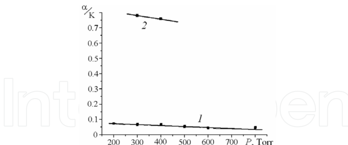
Fig. 20. The dependence of the normalized sound absorption coefficient on the pressure.
