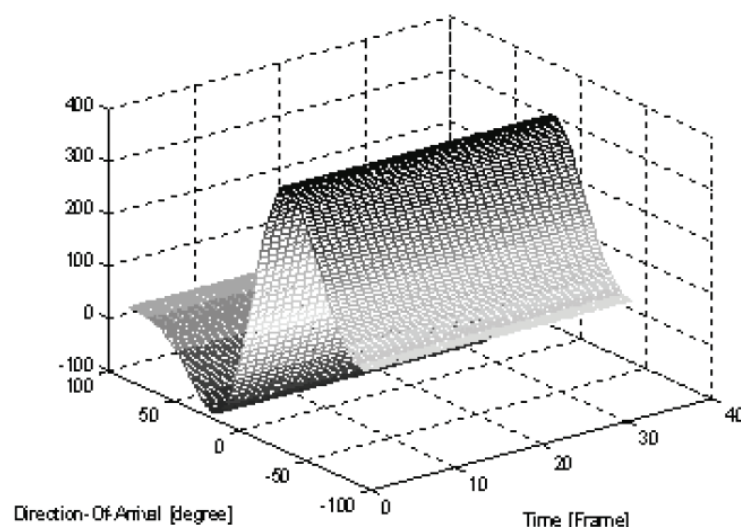
Fig. 2. Waterbed Effect in the DOA Estimation
