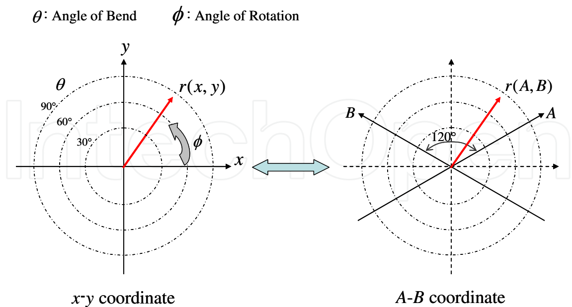
Fig. 18. Change of coordinates
