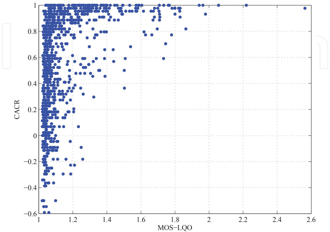
Fig. 8. MOS estimation of DRT words using PESQ (white noise)
