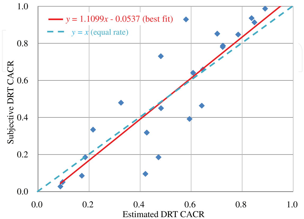
Fig. 11. Subjective CACR vs. estimated CACR (pooled for each feature, female speech with white noise)
