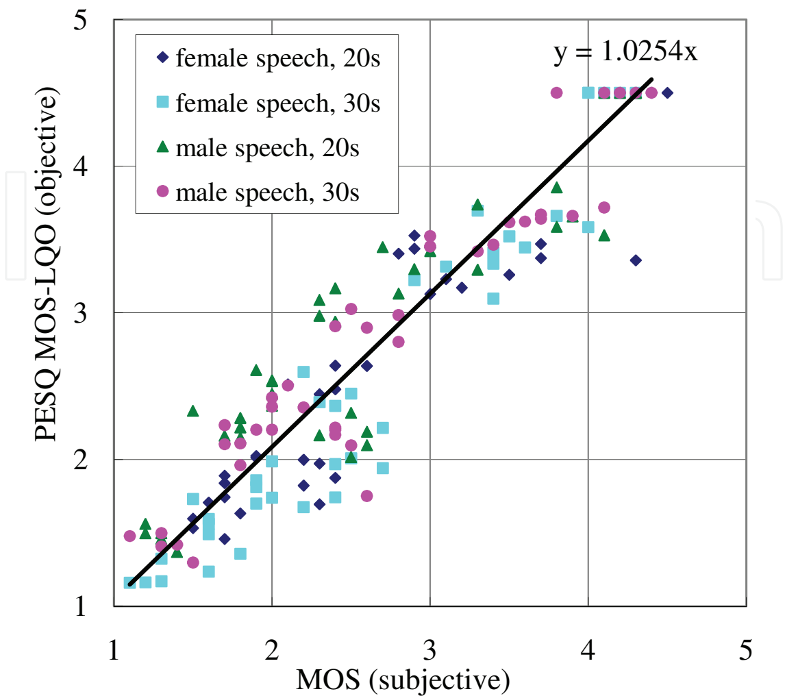
Fig. 7. Example MOS estimation using PESQ
