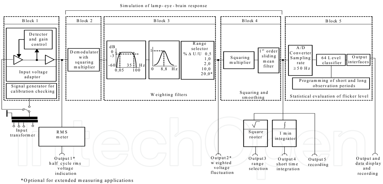
Fig. 3. General layout
