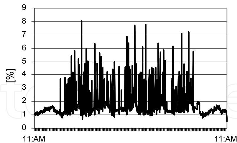
Fig. 19. Variation of THDV values on phase A
