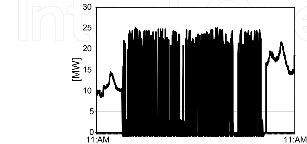
Fig. 15. Variation of the real power at PCC (HV level)
