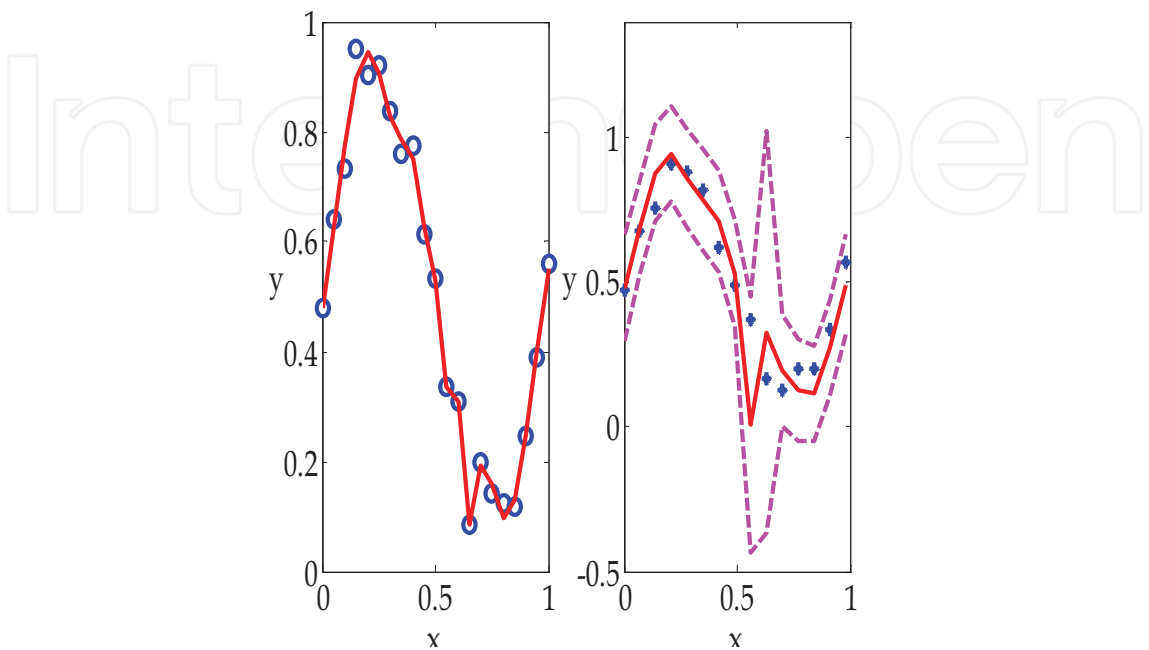
Fig. 4. Neural model of f(x) with five hidden nodes. Left figure: circles - training data; solid line - neural network output. Right figure: asterisks - testing data; solid line - neural network output; dashed lines - 95% confidence interval.
