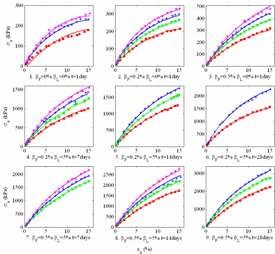
Fig. 5. Relationship of \sigma_a vs. \epsilon_a with different confining pressures (CP) (Experiment data: Symbols with CP values: ■50 kPa, ▼100 kPa, *150 kPa,★200 kPa; The outputs of the neural network are in solid lines)
