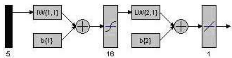
Fig. 13. Diagram of implemented Neural Model
