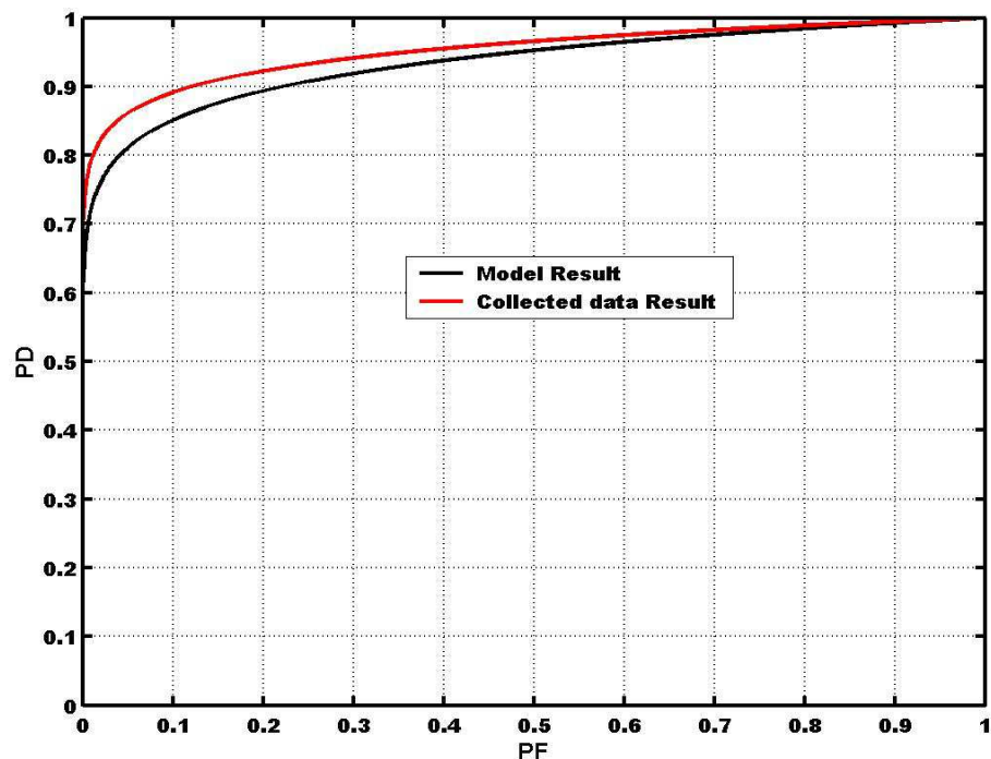
Fig. 9. ROC curves for Vulgar diagnosis Explanation: In figures 7, 8 and 9, it can be seen that the model results compared satisfactorily well with the collected data results for all cases examined in the paper.
