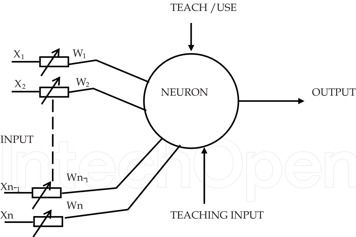
Fig. 2. The neuron model The units of most types of neural networks are organized in layers, which are called input layer, hidden layers(s) and output layer, depending on their functionality. A neural network with n units in its input layer and m units in its output layer, implements a mapping f: X^n \rightarrow Y^m . The sets X^n \subseteq R^n and Y^m \subseteq R^m are the input and output domains. Hidden layers add to the complexity of a neural network, and are important, if arbitrary mappings have to be
