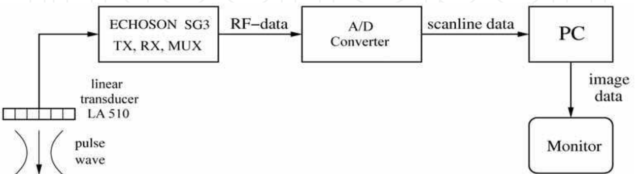
Fig. 11. Block diagram of the ultrasound imaging system
