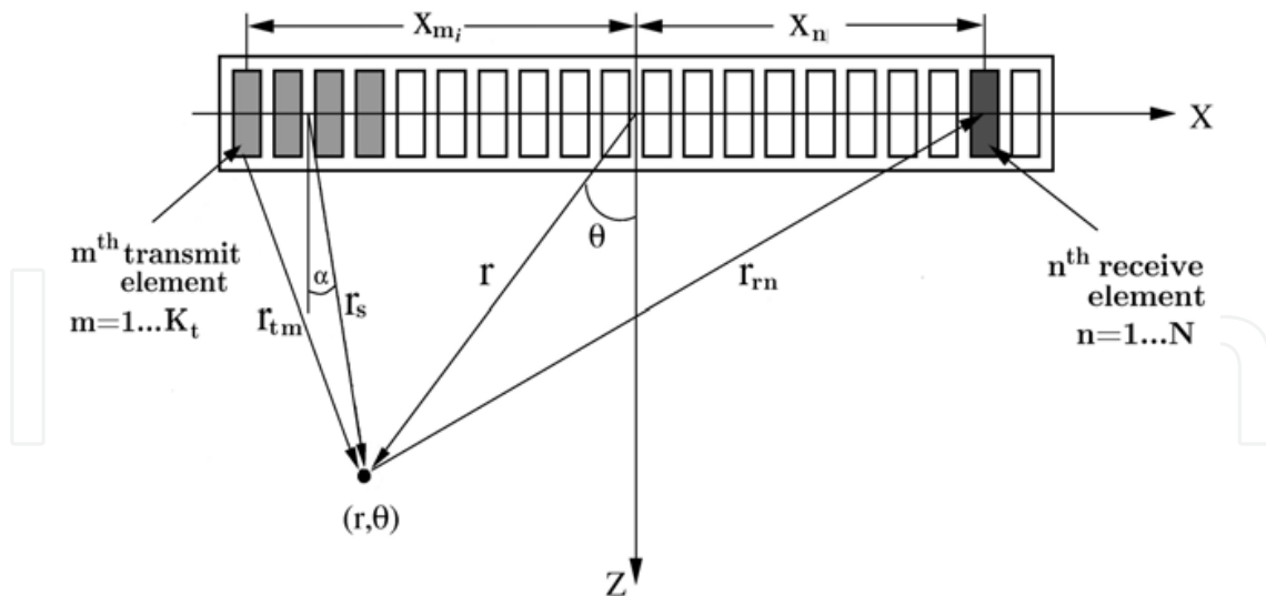
Fig. 4. Geometric relation between the transmit and receive element combination and the focal point
