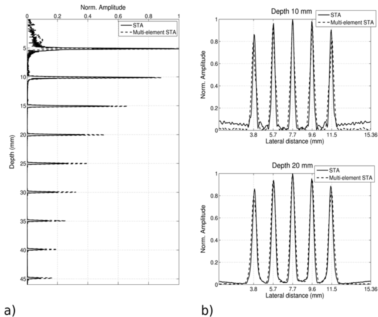
Fig. 10. Comparison of the cross sections between STA method and multi-element STA method: a) axial cross section of the centre line; b) lateral cross section in depth 10 mm (top) and depth 20 mm (bottom)
