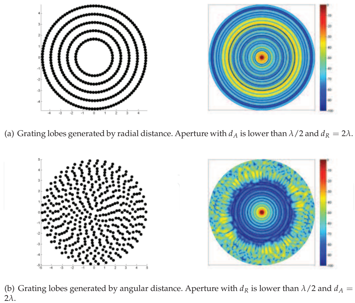
Fig. 8. Grating Lobe generation in Circular Apertures and main distances between elements.
