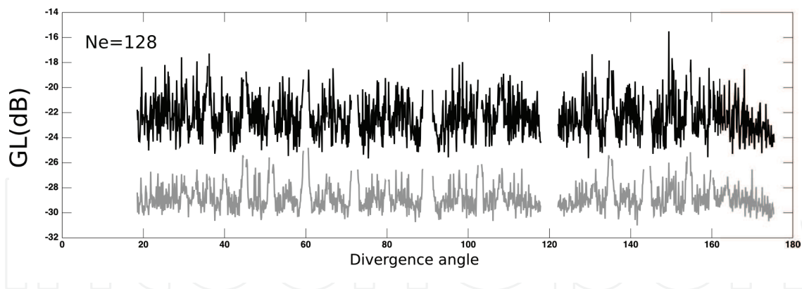
Fig. 4. Narrowband Grating lobe distribution per divergence angle. Black line represents the echo-pulse response if \Delta\alpha = 0^{\circ} ; the gray line represents the echo-pulse response of the better case obtained when \Delta\alpha > 0^{\circ} .
