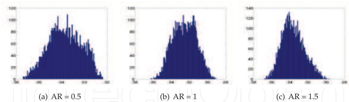
Fig. 10. Distribution of grating Lobe values for 1000 different apertures wideband (60%). The three aspect ration are considered.
