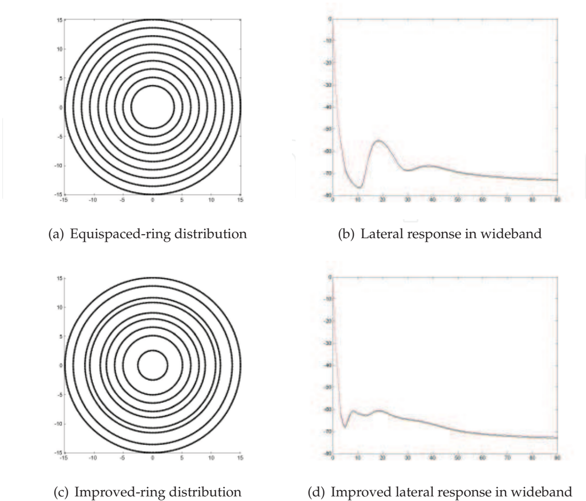
Fig. 11. Improved ring distribution to reduce radial grating lobes
