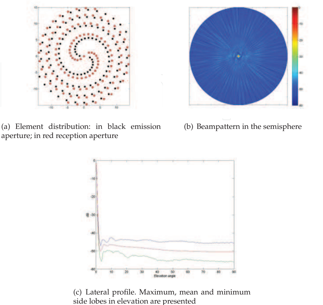
Fig. 6. Best result for SP(28,128) is presented, \alpha = 174.525^\circ .
