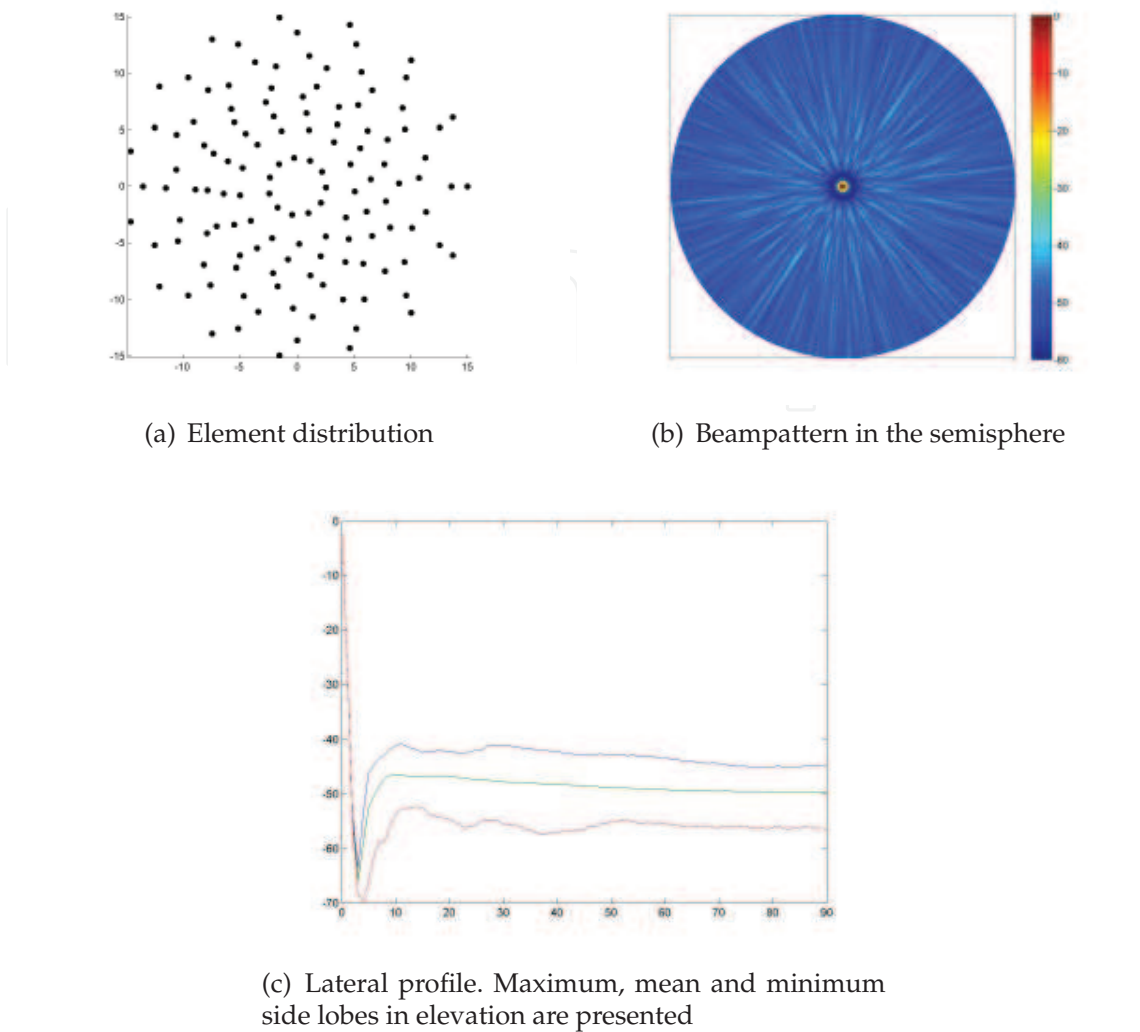
Fig. 12. Best result for CA(128) is presented.
