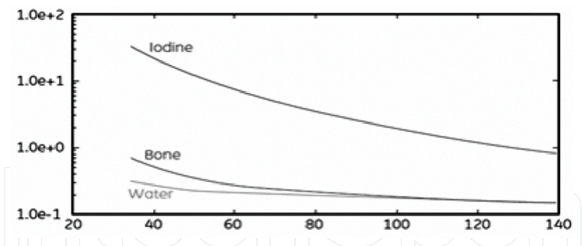
Fig. 2. The bone attenuation curve is a linear combination of iodine and water X-ray; x-axis, photon energy, Kev; y-axis, mass attenuation coefficient, m²/Kg (from D.A.Langan, (Langan DA 2008)
