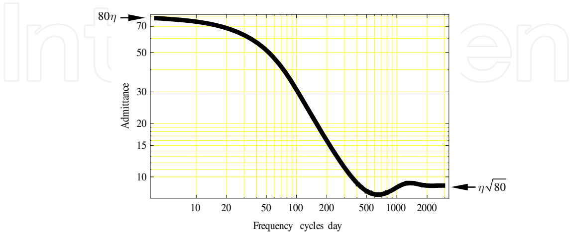
Fig. 9. Admittance for Horns Rev offshore wind farm for 10 m/s and wind direction aligned with the turbine rows.
