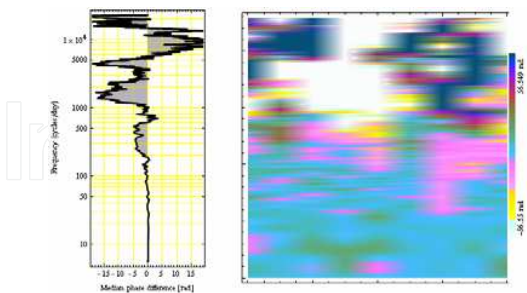
Fig. 20. Estimated phase delay between the power oscillations at the turbine and at the wind farm output. The median value for each frequency f is presented on the left and the phase differences of the spectrograms in Fig. 15 and Fig. 16 are presented on the right. A phase unwrapping algorithm has been used to reconstruct the phase from the SFFT .
