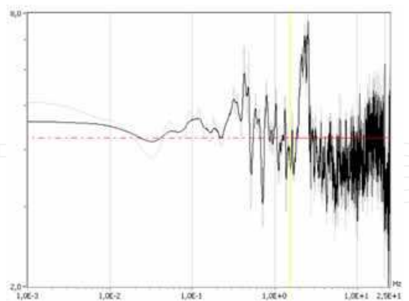
Fig. 14. Admittance of the active power (ratio of the farm PSD to the turbine PSD ). In short, real power oscillations quicker than one minute can be considered independent among turbines of a wind farm because the PSD due to fast turbulence and rotational effects scales proportionally to the number of turbines.
