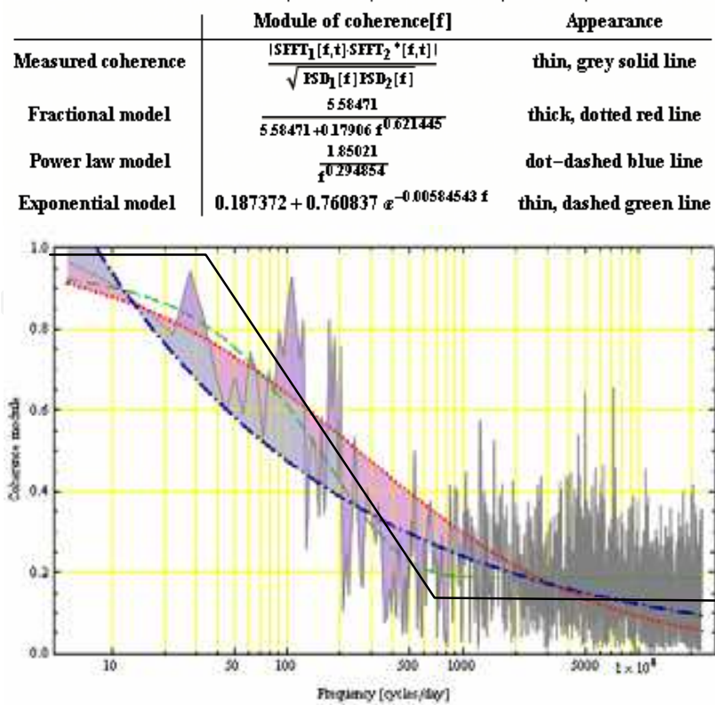
Fig. 18. Coherence models estimated by WINDFREDOM software.
