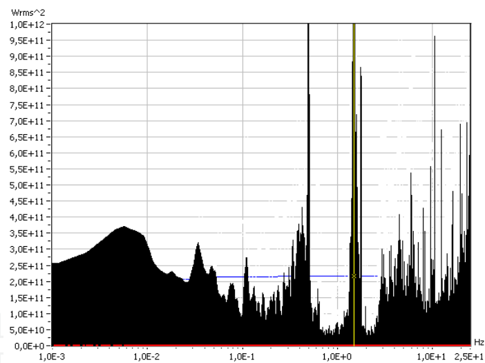
Fig. 8. Contribution of each frequency to the variance of power computed from Fig. 5 (the area bellow f \cdot PSD_p+(f) in semi-logarithmic axis is the variance of power).
