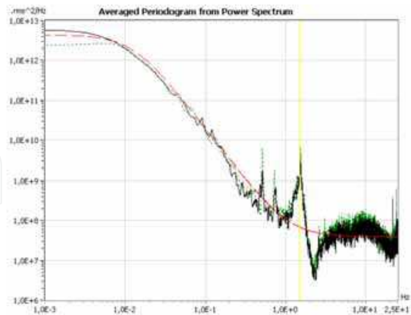
Fig. 13. PSD_{P_{farm}}^{+}(f) of a wind farm (in solid black) and PSD_{P_{turbine}}^{+}(f) of one of its 648 kW turbines times 18 (in dashed green), for time series #1. There is a peak in Fig. 14 at 2\text{ Hz} < f < 2,5\text{ Hz} . The analyzed turbine may have comparative less fluctuations in such range than the other turbines in the farm (the measured turbine may have better adjusted rotor and blades, while others turbines may suffer from more vibration effects). But other feasible reason is a higher correlation degree between the turbines at such frequency band, probably induced by turbine control or voltage variations.
