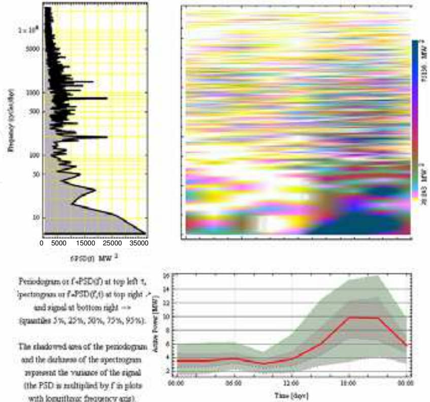
Fig. 15. Spectrogram of the real power [MW] at a turbine (times the turbines in the farm, 27).
