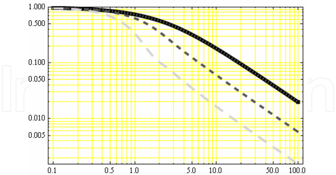
Fig. 11. Normalized ratio H^2(f) for transversal a \ll b (solid thick black line) and longitudinal a \gg b areas (dashed dark gray line for A_{long} = 4 , long dashed light gray line for A_{long} = 1,8 ). Horizontal axis is expressed in either longitudinal or lateral adimensional frequency a A_{long} f / \langle U_{wind} \rangle or b A_{lat} f / \langle U_{wind} \rangle .
