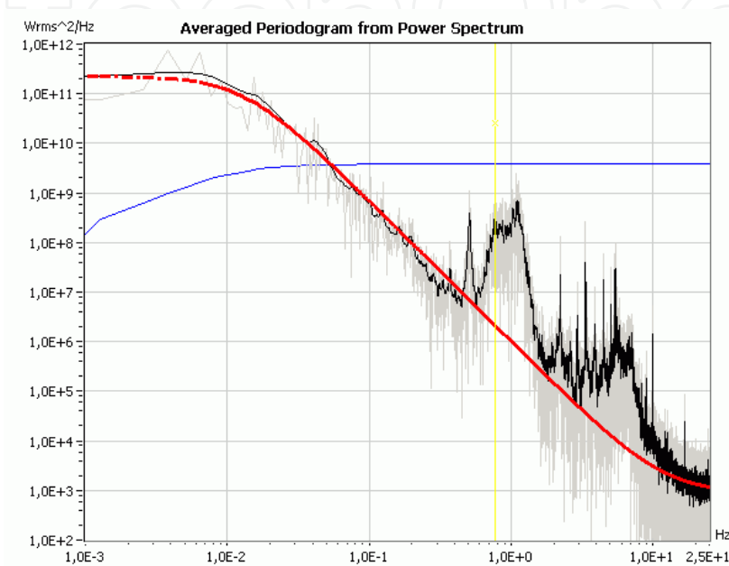
Fig. 3. PSD_{p+}(f) parameterization of active power of a 750 kW wind turbine for wind speeds around 6,7 m/ s (average power 190 kW) computed from 13 minute data. The signal in the time domain can be computed from the inverse Fourier transform:
