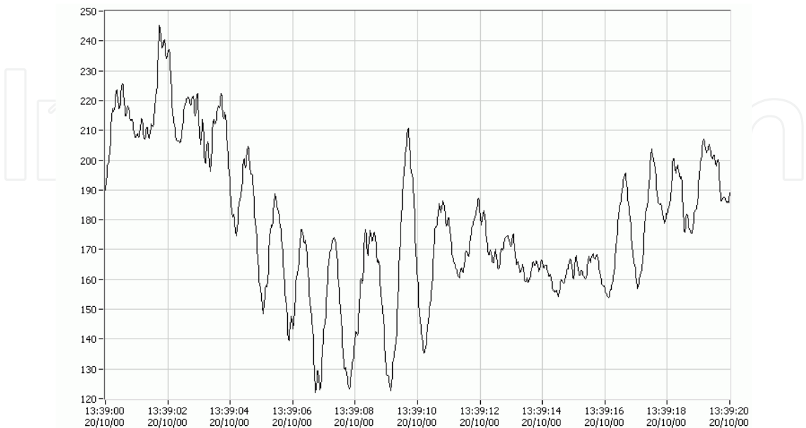
Fig. 1. Active power of a 750 kW wind turbine for wind speeds around 6,7 m/ s during 20 s.
