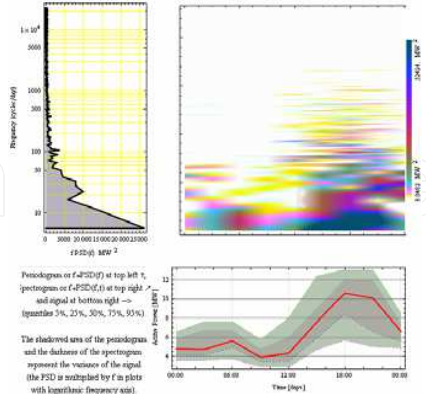
Fig. 16. Spectrogram of the real power [MW] at the substation.
