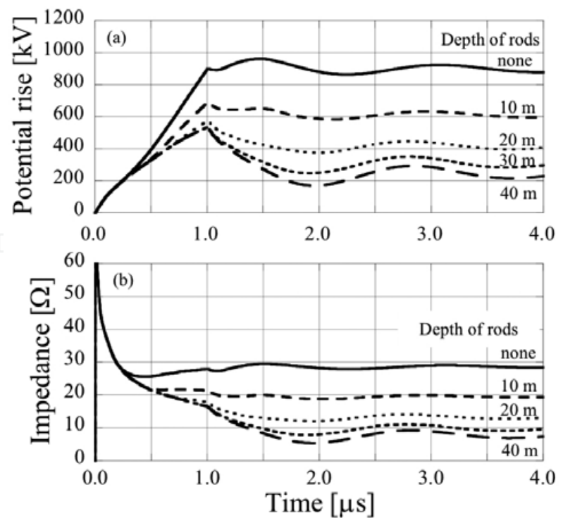
Fig. 9. Transient waveforms of Model (b): foundation with vertical rods. (upper graph: earth potential rise, lower graph: simultaneous impedance)
