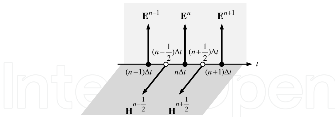
Fig. 4. Arrangement of the electric field E and magnetic field H in the time difference domain Eqs. (10) and (11) can be converted to Eqs. (12) and (13) by difference approximation.
