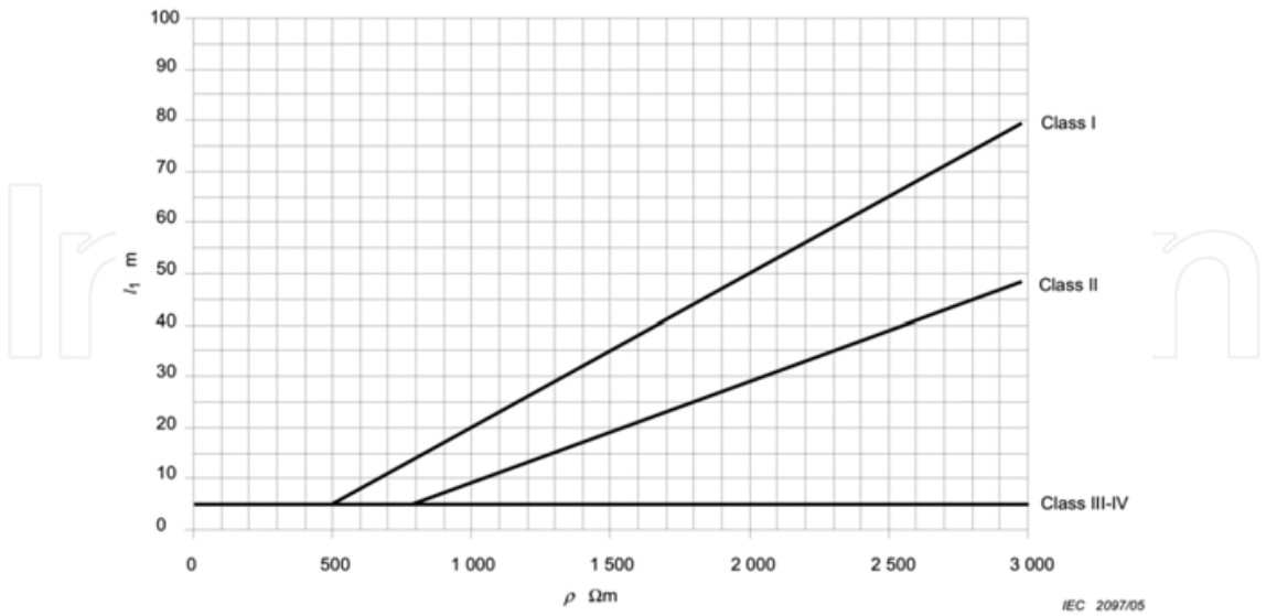
Fig. 3. Minimum length l_1 defined in IEC 62305-3 (from IEC 2006)
