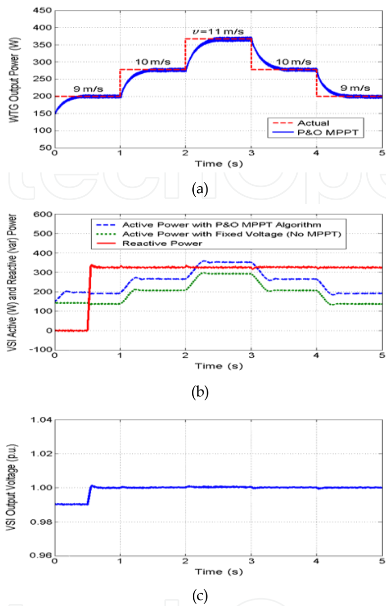
Fig. 16. Simulation results for simultaneous active and reactive power exchange with the utility distribution grid (APCM and VCM). (a) PMSG generator output power. (b) VSI output active and reactive power. (c) PCC terminal voltage.
