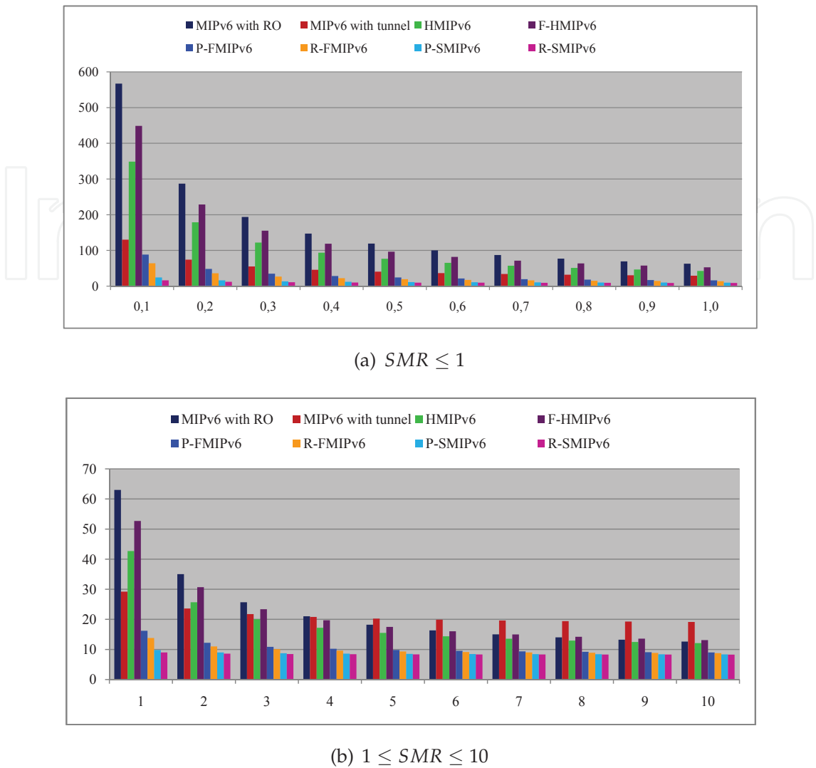
Fig. 10. Total cost vs. SMR for n = 1 tunnel mode (50.80), predictive FMIPv6 (31.63), reactive FMIPv6 (24.60), predictive SMIPv6 (12.89), and reactive SMIPv6 (10.54). In addition, as SMR \geq 1 , the impact of mobility signaling cost on the total cost reduces while packet delivery cost becomes more important over the total cost. The higher the SMR, the more important is the packet delivery cost over the total cost. As a result, when SMR \geq 5 , MIPv6 with tunnel mode requires the highest cost than other protocols. The total cost on average in descent order is MIPv6 with RO mode (23.40), F-HMIPv6 (21.57), MIPv6 with tunnel mode (21.28), HMIPv6 (18.64), predictive FMIPv6 (10.54), reactive FMIPv6 (9.84), predictive SMIPv6 (8.67), and reactive SMIPv6 (8.43). Such values are shown in Figure 10.b. Besides, SMIPv6 yields the best performance amongst all schemes, due to lower signaling cost and no additional processing cost at the MAP. Figures 11.a and 11.b also illustrate the variation of total cost as the average session-to-mobility ratio changes for MAP domains with four rings, using the random-walk model. The total cost decreases as the SMR augments, the same observation applies to Figures 10.a and 10.b. Besides, increasing the MAP domain size leads to a reduction of total cost for HMIPv6 and F-HMIPv6, yet no impact on MIPv6, FMIPv6 and SMIPv6 protocols.
