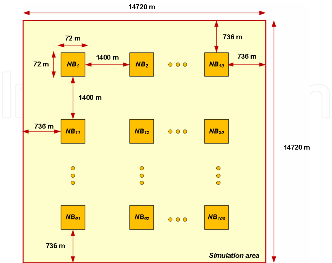
Fig. 7. Simulation layout
