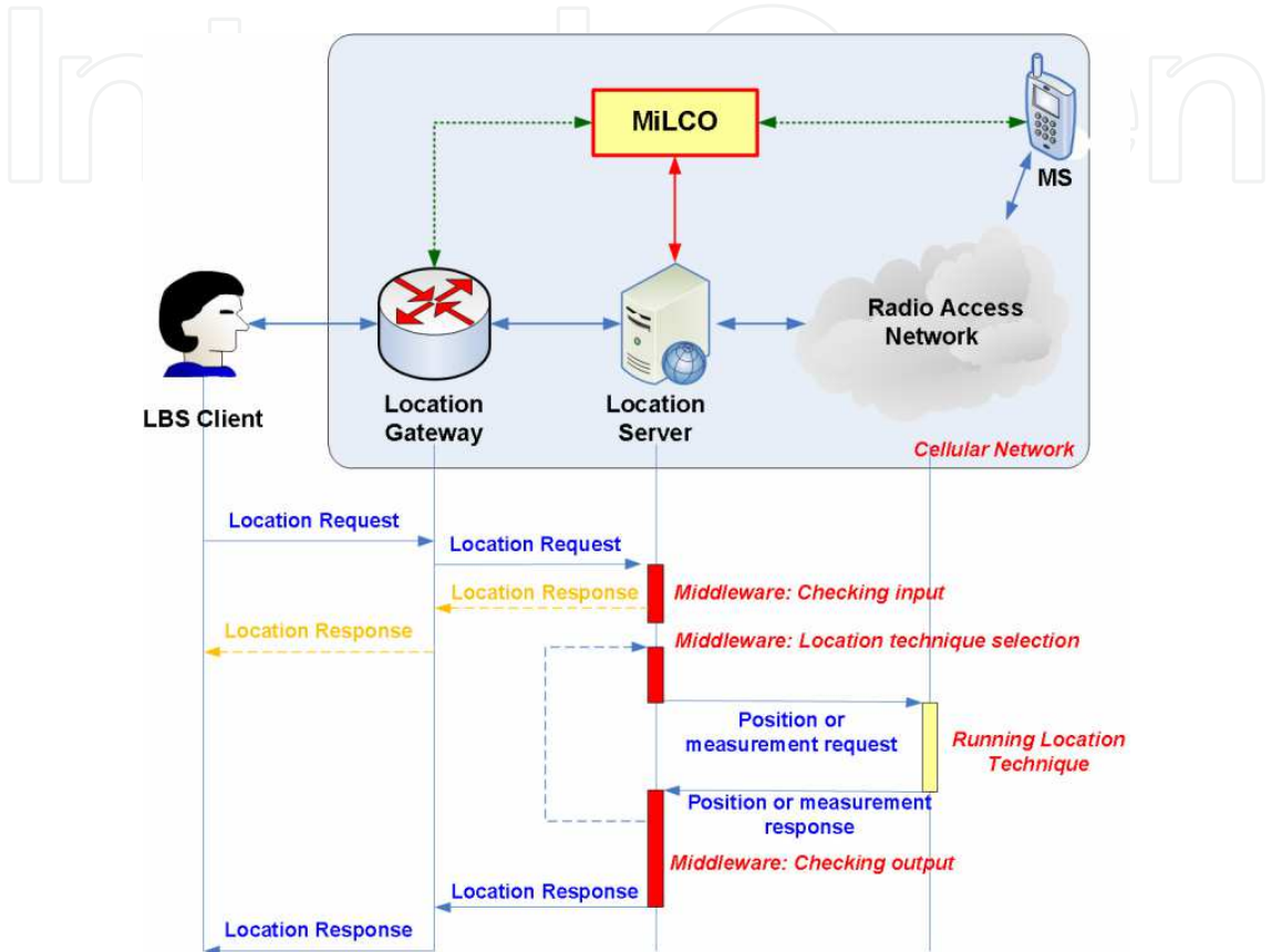
Fig. 4. MILCO system architecture
