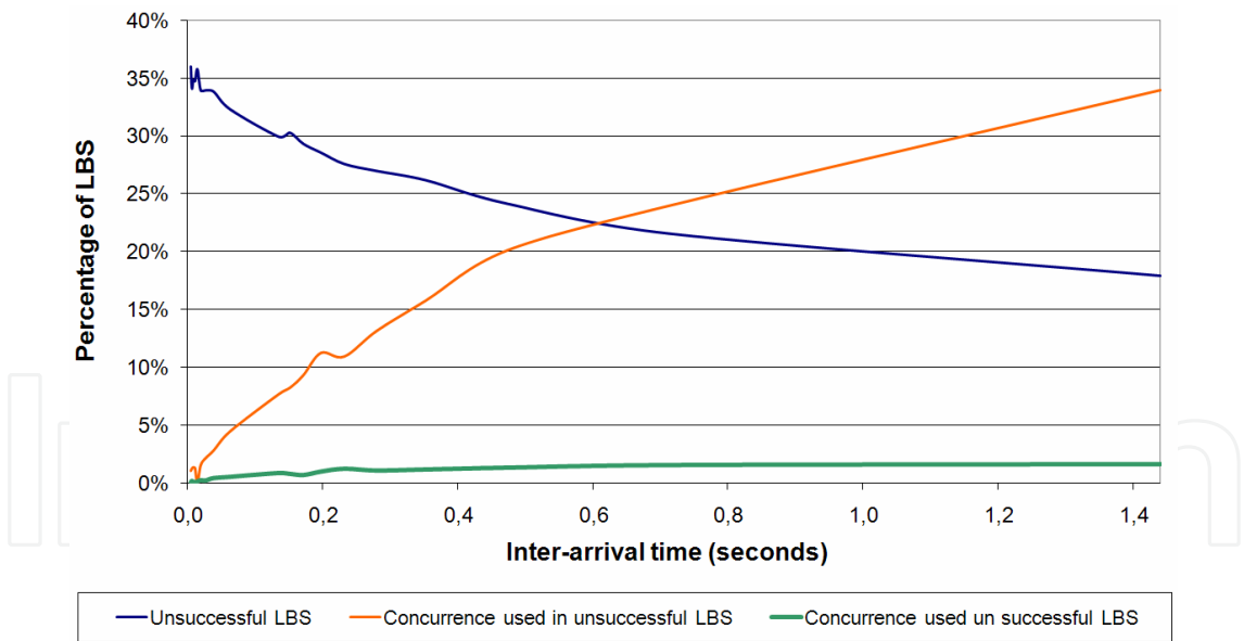
Fig. 11. Performance of the concurrence module
