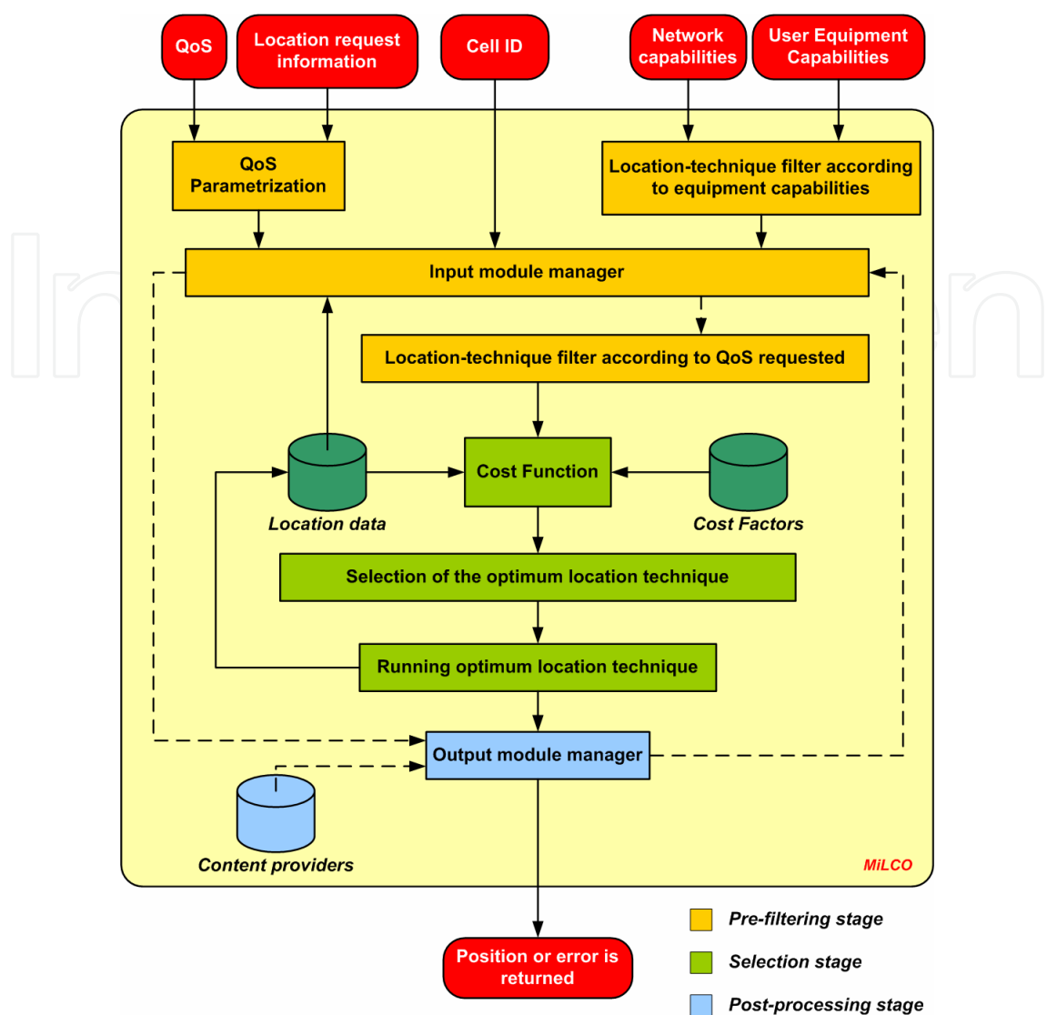
Fig. 5. Block diagram of MILCO
