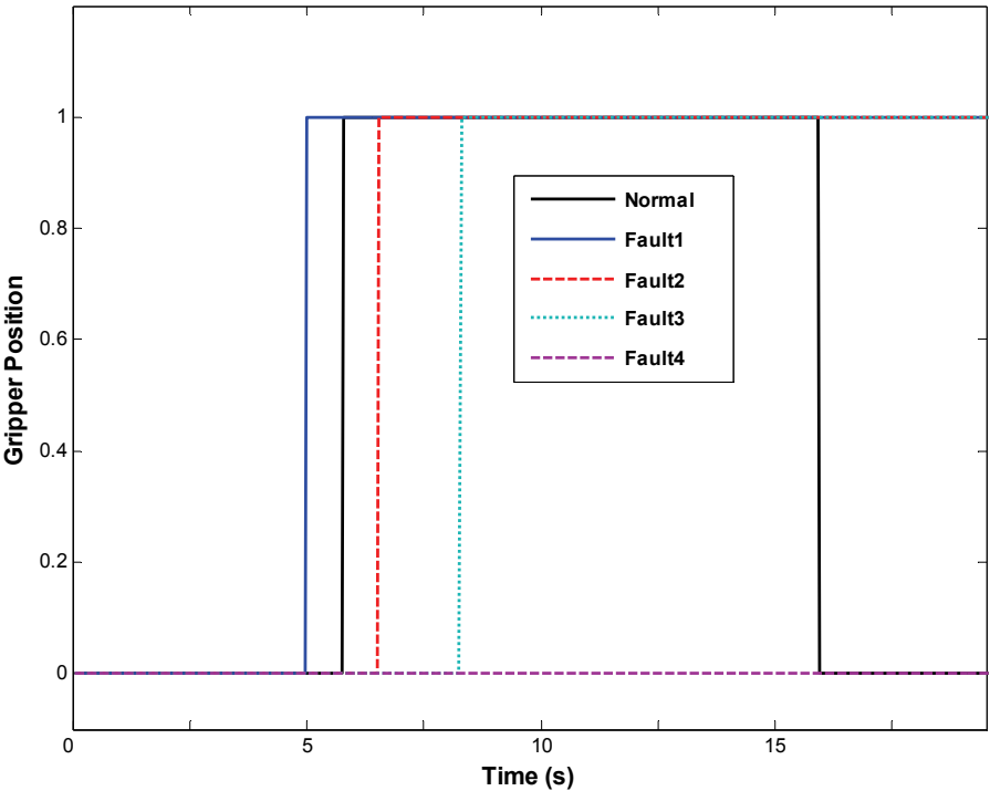
Fig. 4. Gripper Pick
