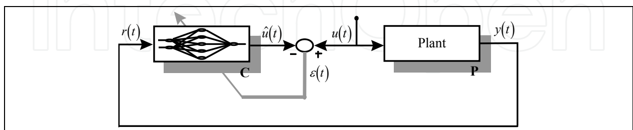
Fig. 5. Inverse plant modelling
