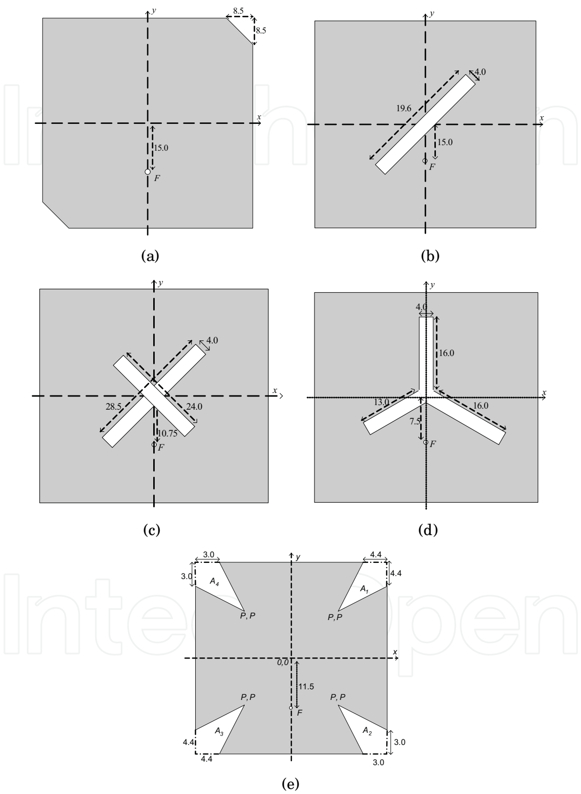
Fig. 2. Slotted/ slit-microstrip patch structures for CP; (a) Antenna#1, (b) Antenna#2, (c) Antenna#3, (d) Antenna#4 and (e) Antenna#5.
