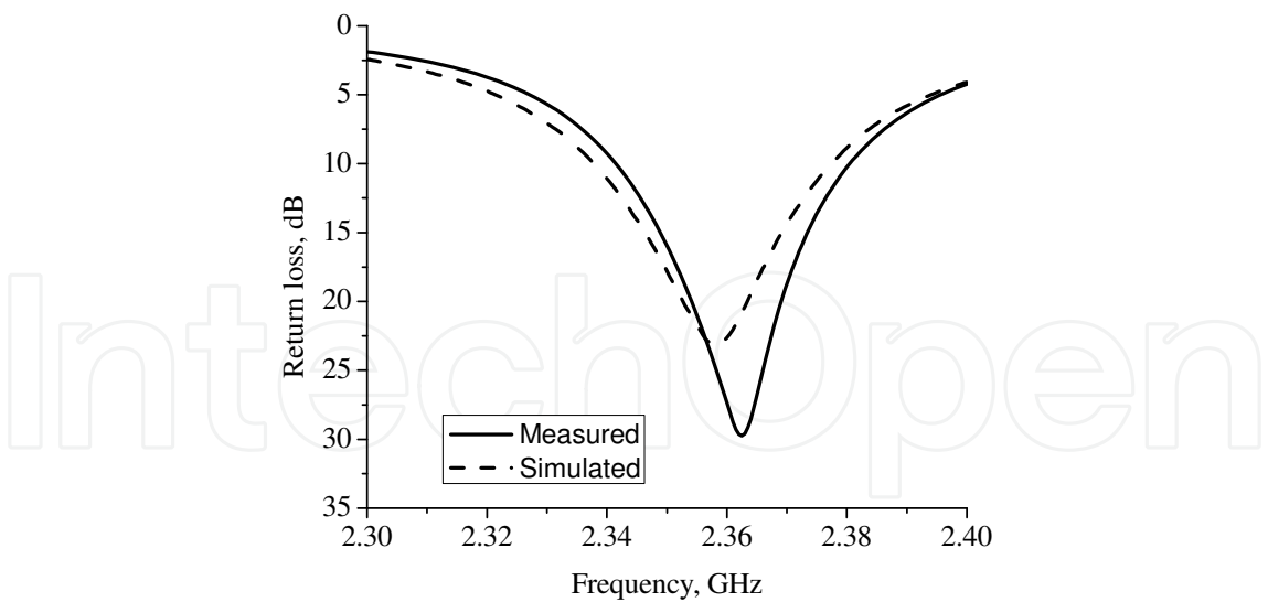
Fig. 10. (a). Simulated and measured return loss of the symmetric-slit with rectangular slot patch antenna.
