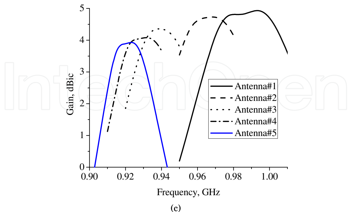
Fig. 3. Simulated performances of the CP slotted/ slit-microstrip antennas; (a) return loss, (b) axial-ratio at the boresight and (c) gain at the boresight.
