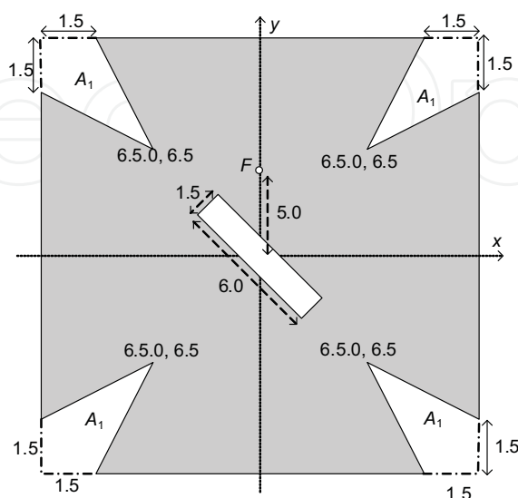
Fig. 9. V-shaped symmetric-slit with rectangular-slot patch radiator.
