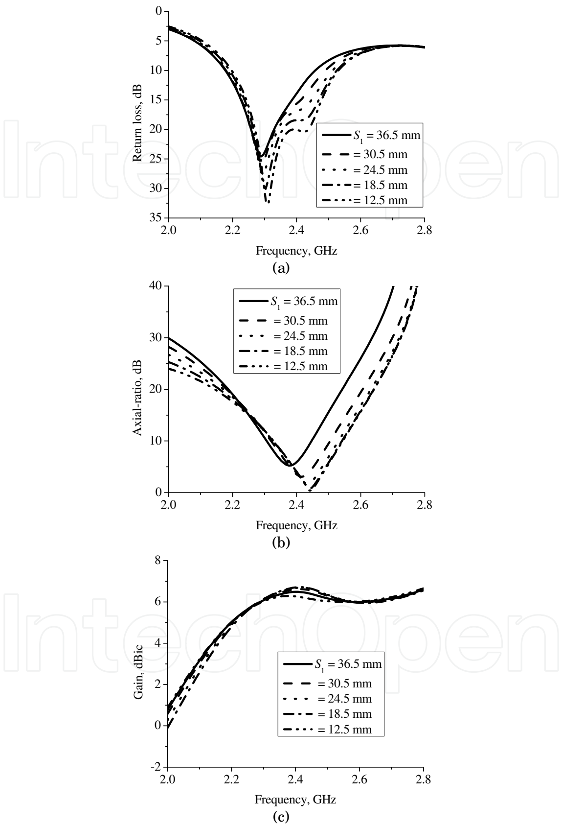
Fig. 13. Effect of the S_1 on antenna parameters of Z-shaped slot antenna; (a) return loss, (b) axial-ratio at the boresight and (c) gain at the boresight.
