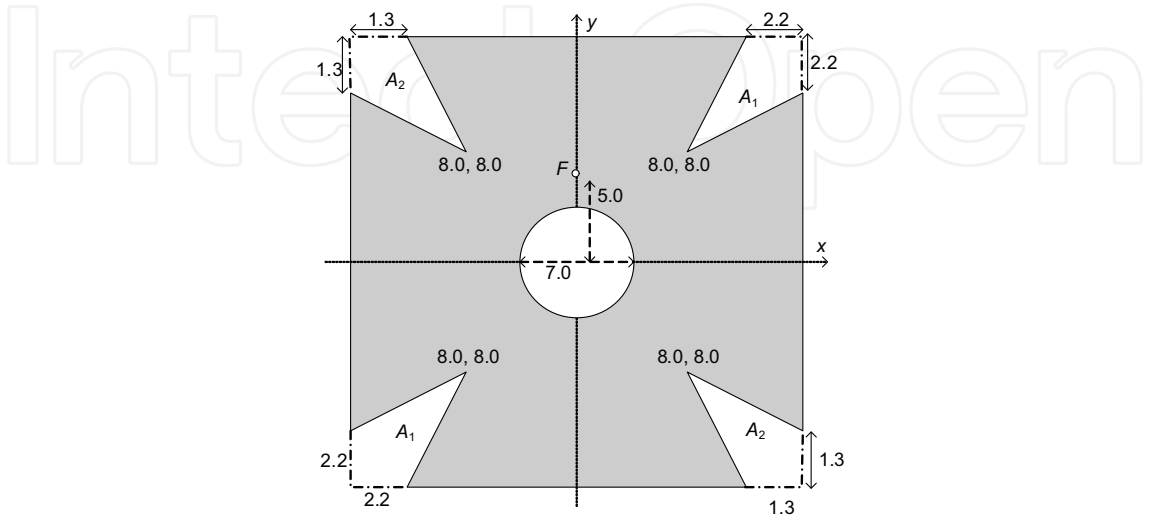
Fig. 6. Symmetric-slit with circular-slot patch radiator.
