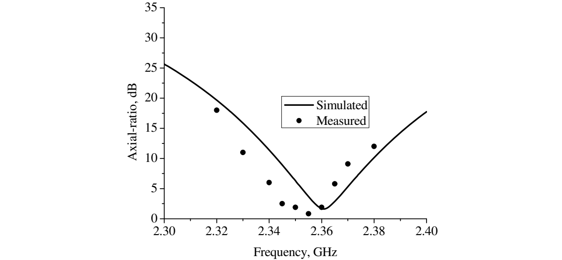
Fig. 10. (b). Simulated and measured axial-ratio at boresight of the symmetric-slit with rectangular slot patch antenna.
