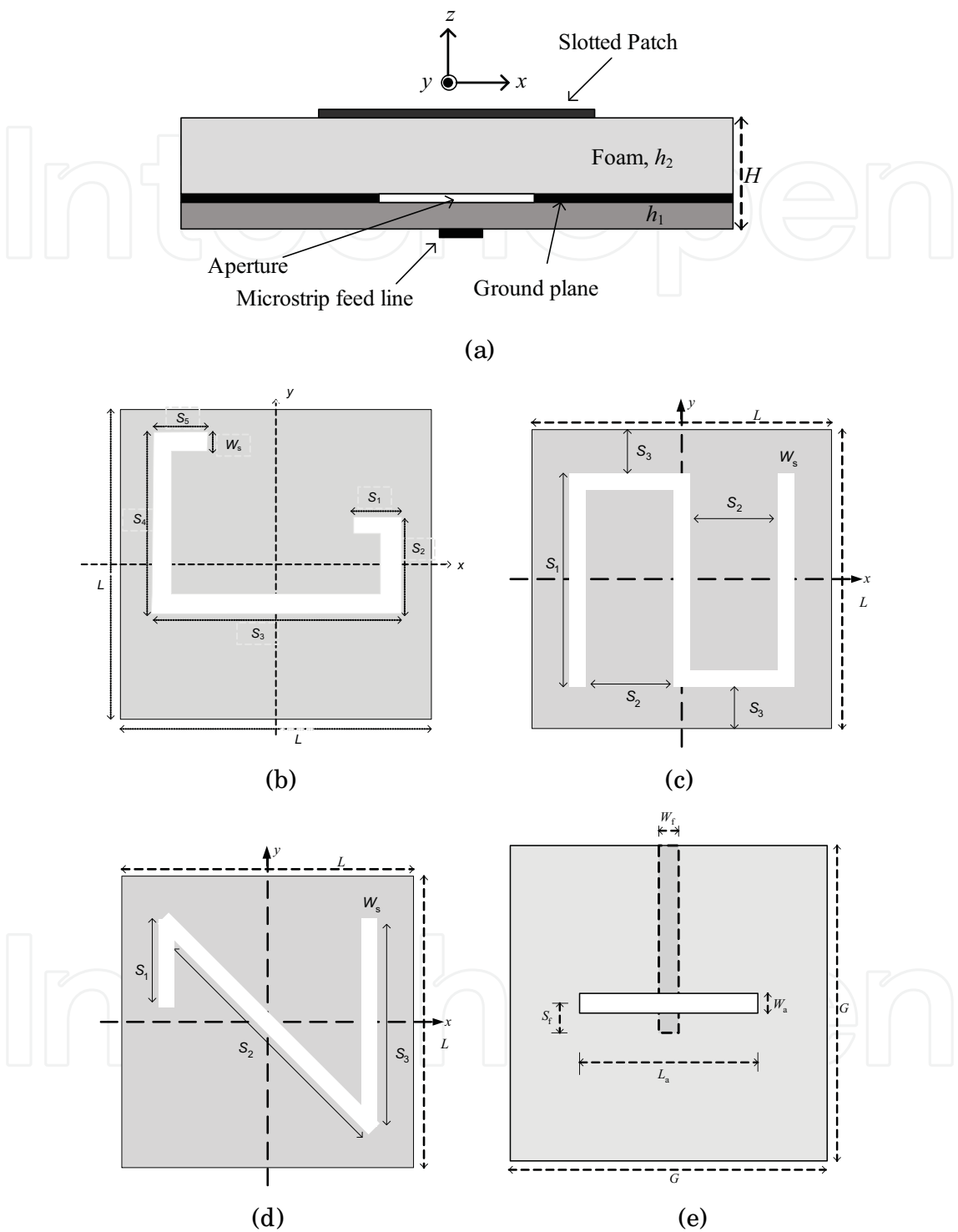
Fig. 11. Aperture-coupled CP slotted microstrip antenna; (a) cross-section view, (b) C-shaped slotted patch, (c) S-shaped slotted patch, (d) Z-shaped slotted patch, and (e) aperture-coupled feed structure.
