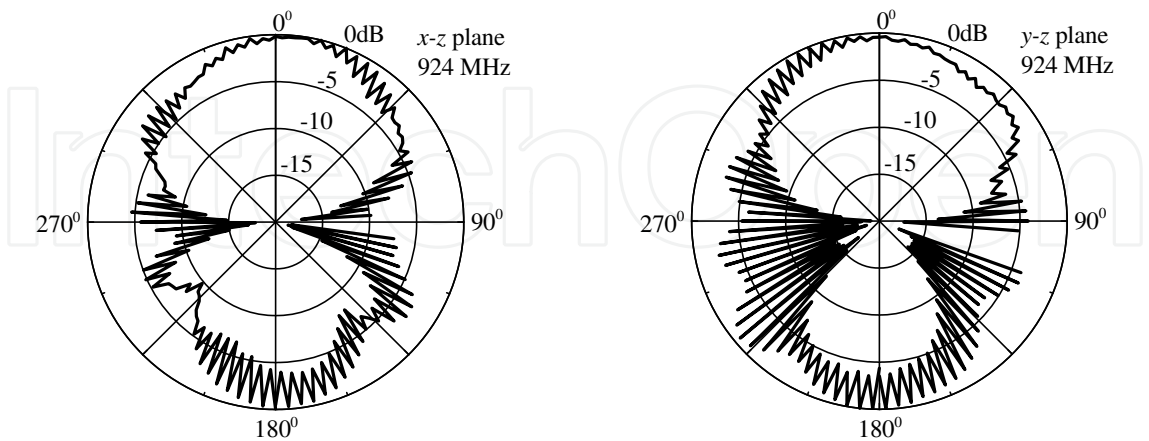
Fig. 5. Measured radiation patterns at 924 MHz.
