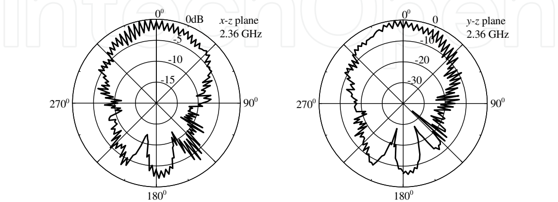
Fig. 10. (c). Measured radiation patterns in x - z and y - z planes at 2.36 GHz of the symmetric-slit with rectangular slot patch antenna
