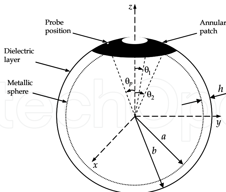
Fig. 1. Geometry of a probe-fed spherical-annular microstrip antenna.
