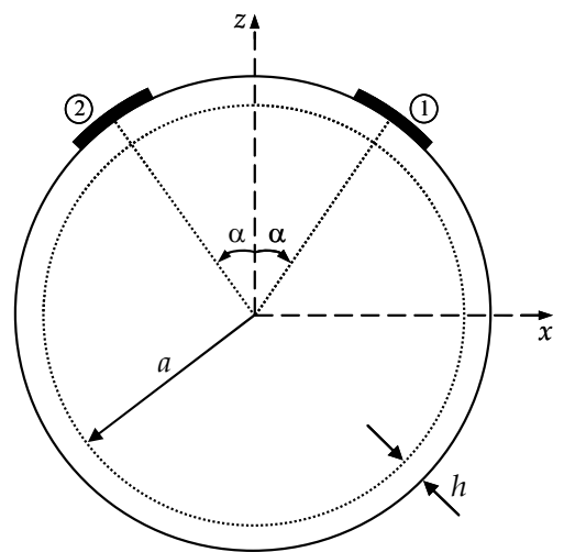
Fig. 14. Two-element array: cut in xz -plane.
