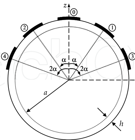
Fig. 18. Five-element array: cut in xz plane.
