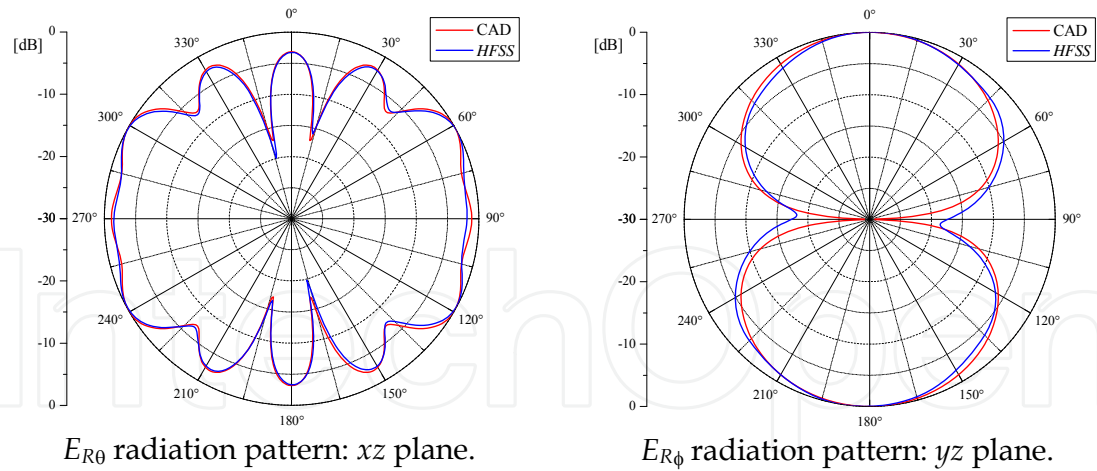
Fig. 16. Two-element array radiation patterns: \alpha = 90^\circ .
