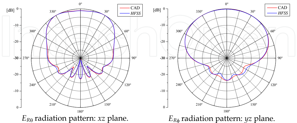
Fig. 19. Five-element array radiation patterns.
