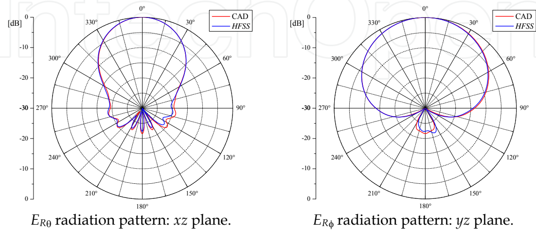
Fig. 15. Two-element array radiation patterns: \alpha = 15^\circ .
