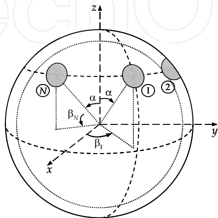
Fig. 20. Circumferential-spherical array.
