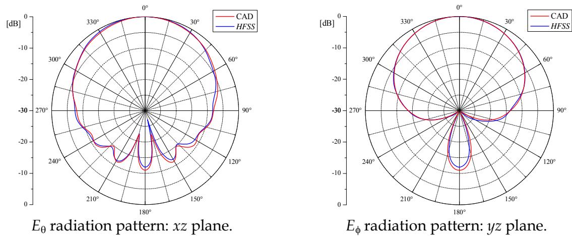
Fig. 25. Radiation patterns.
