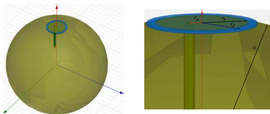
Fig. 23. Faceted antenna geometry.
