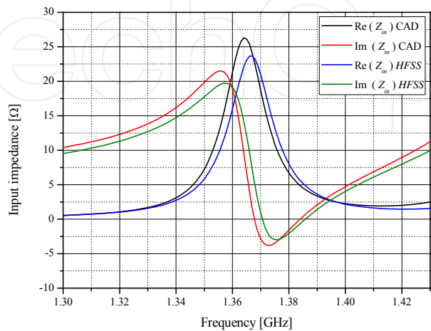
Fig. 11. Spherical-annular antenna input impedance ( \text{TM}_{10} mode).
