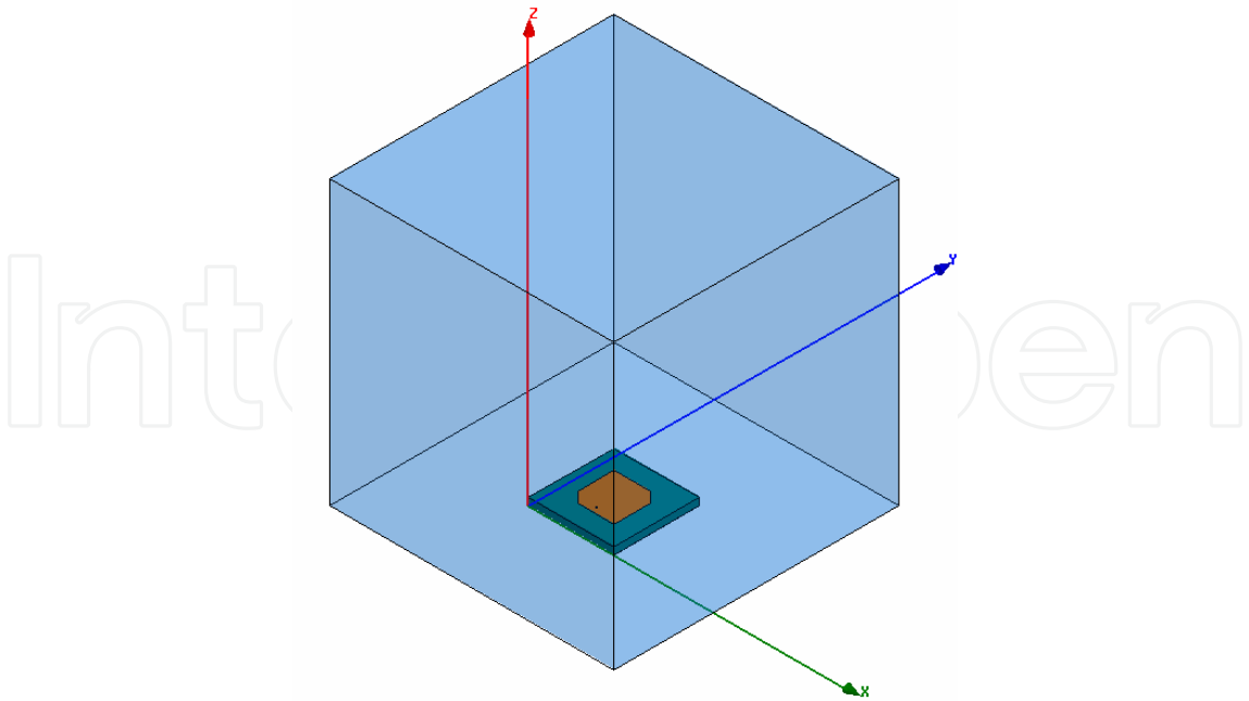
Fig. 35. Geometry of the Wheeler cap simulation through the HFSS package.
