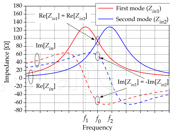
Fig. 11. Impedances of the fundamental modes: standard design.
