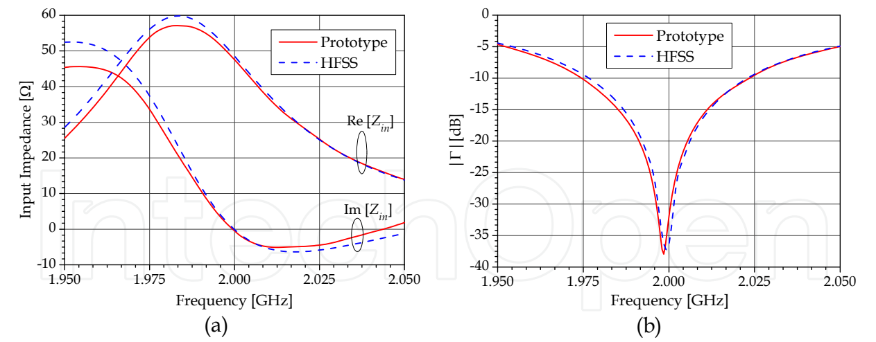
Fig. 27. PIFA antenna: (a) input impedance - (b) reflection coefficient magnitude.
