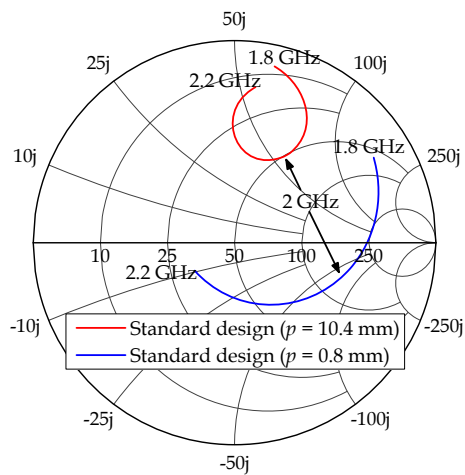
Fig. 5. Input impedances: standard design.
