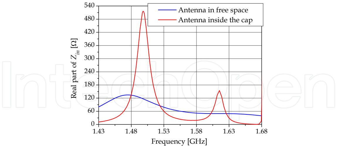
Fig. 36. Low-cost Glonass antenna: real part of its input impedance.
