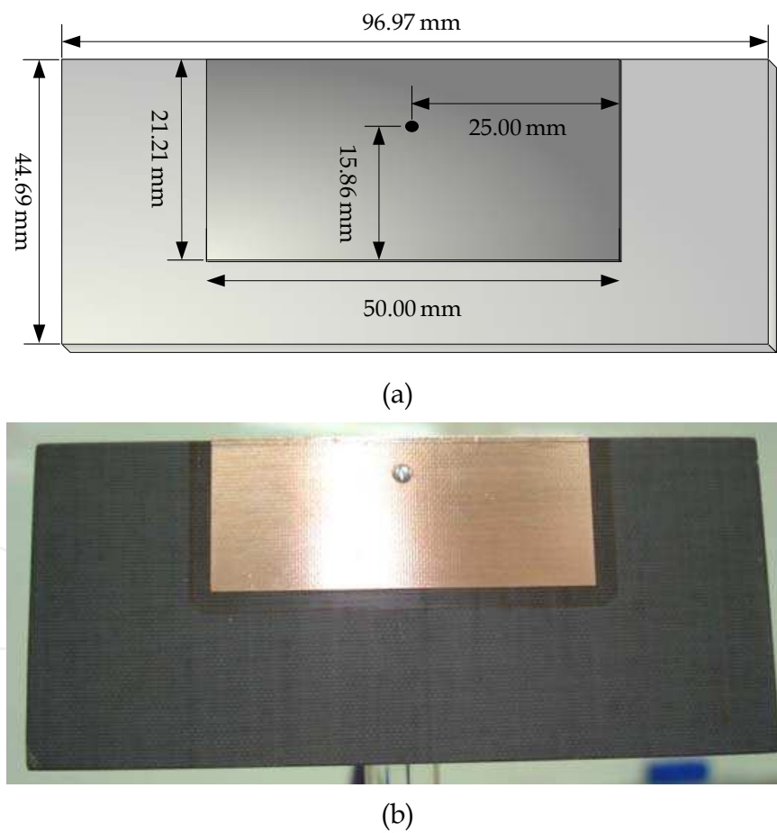
Fig. 26. PIFA antenna: (a) geometry - (b) photo of the prototype.
