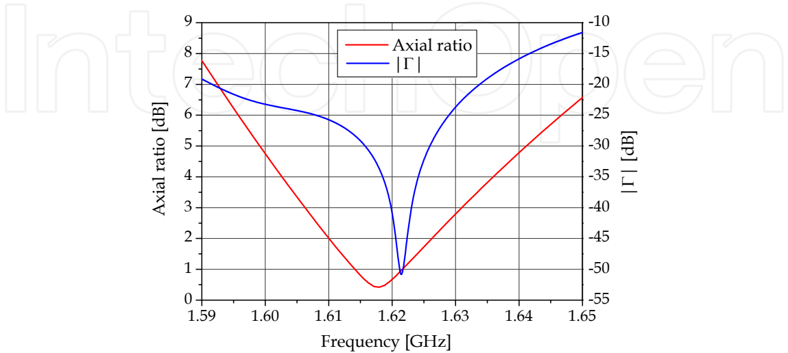
Fig. 31. Globalstar antenna axial ratio and reflection coefficient magnitude: Tx radiator.
