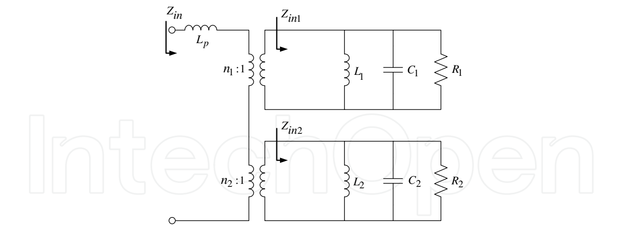
Fig. 10. Equivalent circuit for singly-fed CP microstrip antennas.
