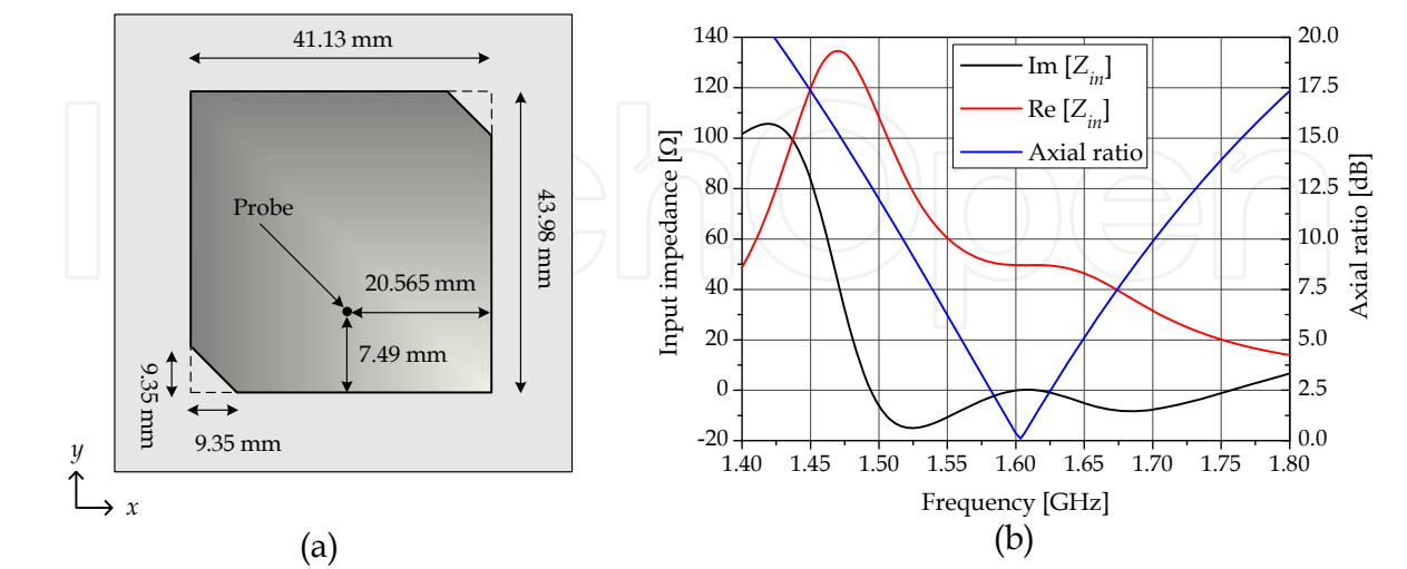
Fig. 28. CP truncated-corner patch: (a) geometry - (b) axial ratio and input impedance.
