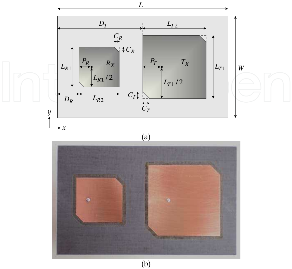
Fig. 30. Globalstar antenna: (a) geometry - (b) photo of the prototype. The axial ratio and reflection coefficient magnitude are presented in Figs. 31 and 32 for the Tx and Rx antennas, respectively.
