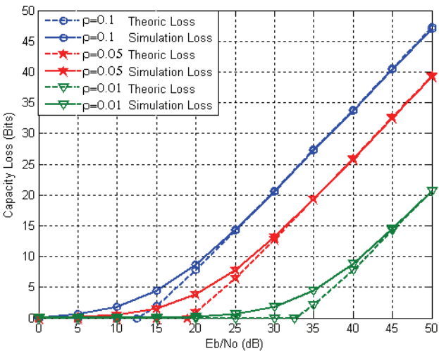
Fig. 9. Capacity loss for K=4 user
