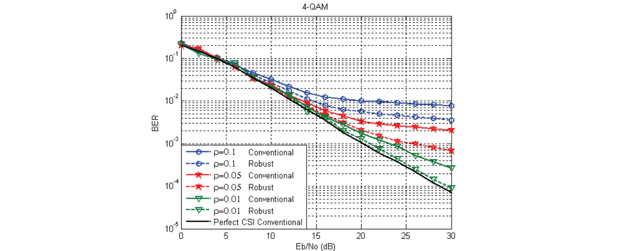
Fig. 11. Robust THP optimization performance
