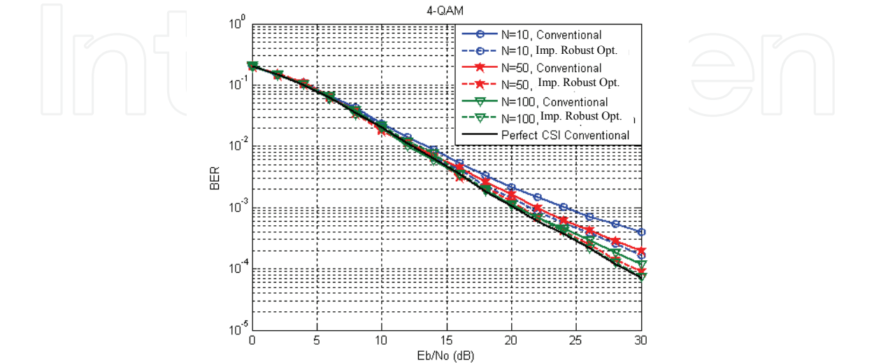
Fig. 12. Improved robust optimization performance with different N value
