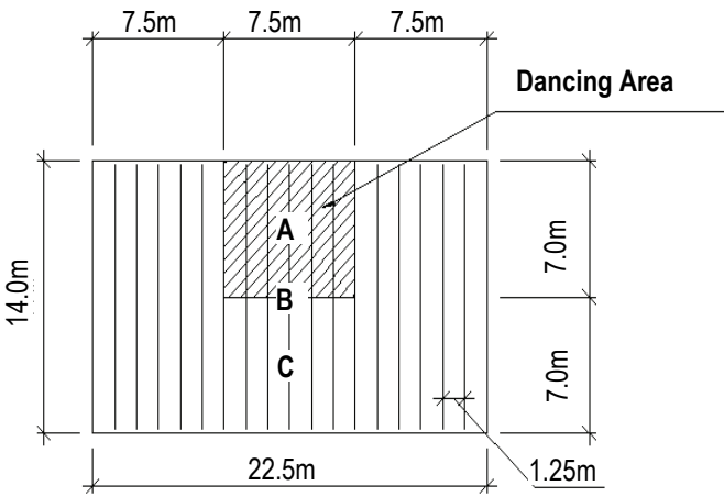
Fig. 3. Dancing floor layout (dimensions in m)
