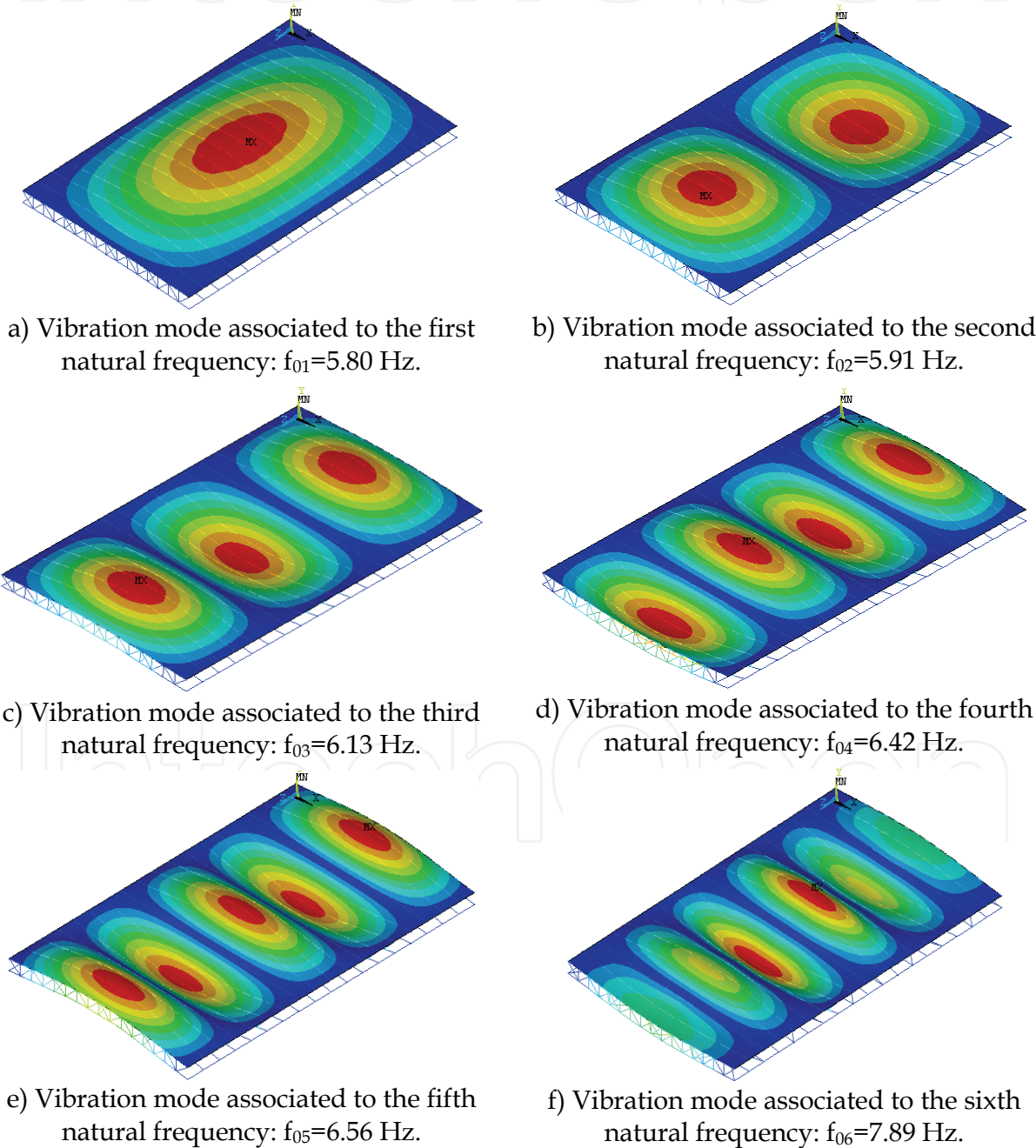
Fig. 9. Composite floor (steel-concrete) vibration modes
