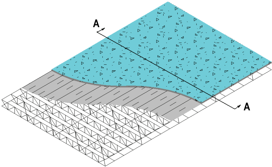
Fig. 4. Structural model three-dimensional view
