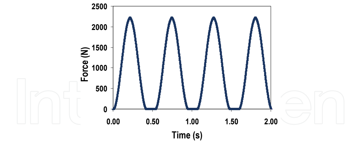
Fig. 2. Dynamic loads induced by dancing associated to the following parameters: T=0.53s, T c =0.43s, T s =0.10, K p =2.78 and CD=1.0
