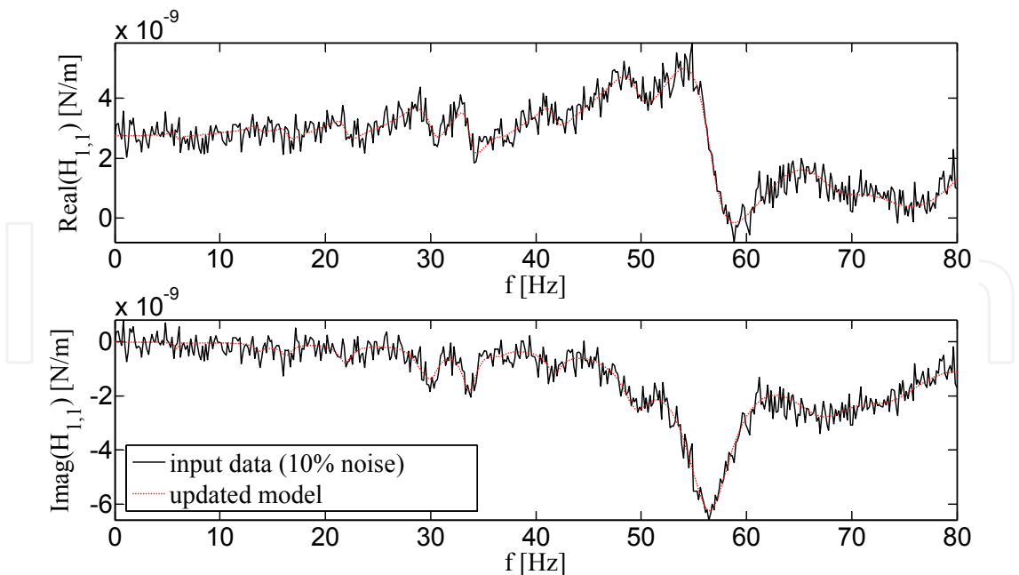
Fig. 21. Comparison of (input point 1; output point 1) FRF considering noise (10% case) after updating (4 measurement response dofs): the input data (black line) and the updated model (red line).
