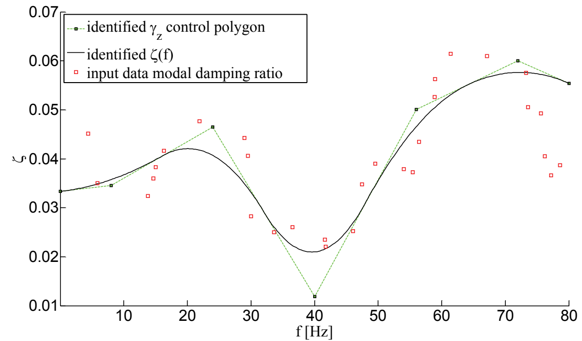
Fig. 8. Comparison of the modal damping ratio used to simulate the measurements (red squares) and the identified \zeta(f) (black line; green filled squares refer to B-spline curve control coefficients). Example with 12 measurement response dofs and without noise.
