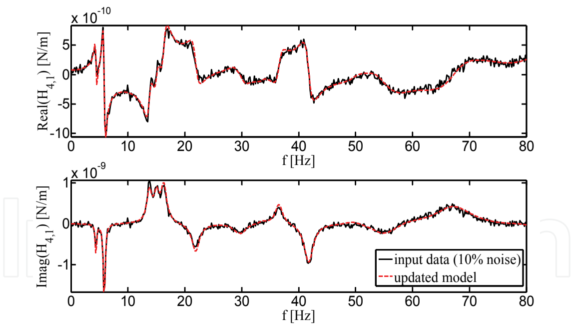
Fig. 22. Comparison of (input point 1; output point 4) FRF considering noise (10% case) after updating (4 measurement response dofs): the input data (black line) and the updated model (red line).
