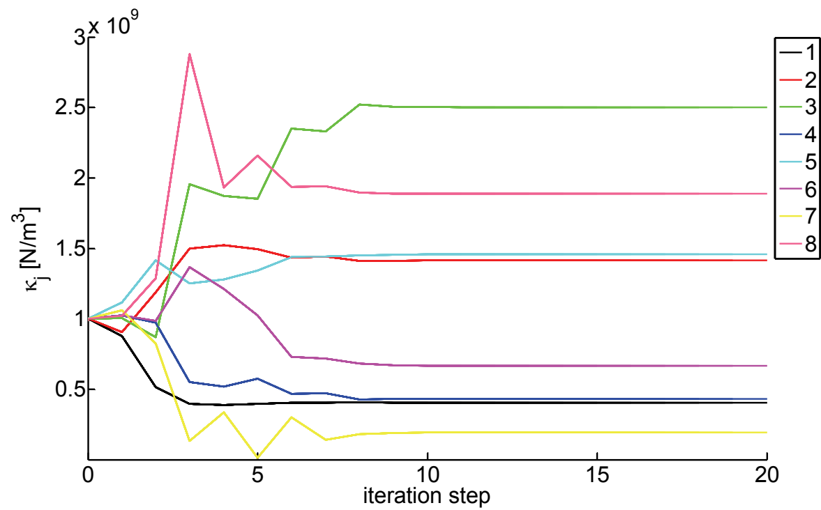
Fig. 6. Evolution of the stiffness parameters \kappa_j ( j=1,...,8 in the legend) during iterations by adopting the proposed updating procedure. Example with 12 measurement response dofs and without noise.
