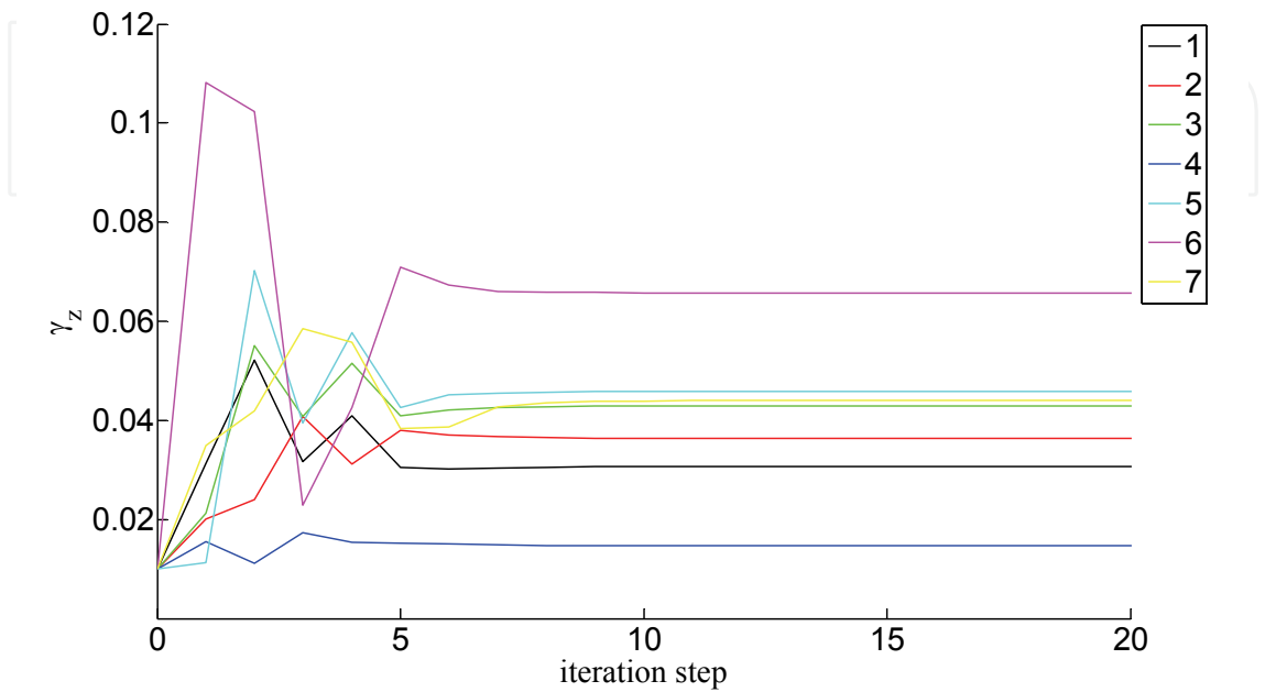
Fig. 15. Evolution of the damping parameters \gamma_z(z=1,...,7 in the legend) during iterations by adopting the proposed updating procedure. Example with 4 measurement response dofs and with 3% noise.
