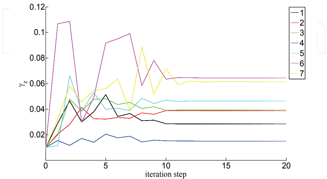
Fig. 19. Evolution of the damping parameters \gamma_z ( z=1,...,7 in the legend) during iterations by adopting the proposed updating procedure. Example with 4 measurement response dofs and with 10% noise.
