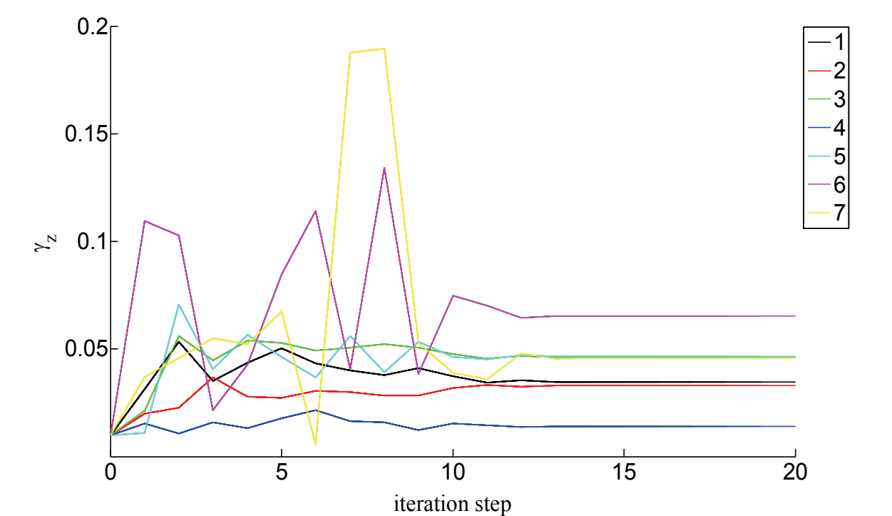
Fig. 11. Evolution of the damping parameters \gamma_z ( z=1, \dots, 7 in the legend) during iterations by adopting the proposed updating procedure. Example with 4 measurement response dofs and without noise.
