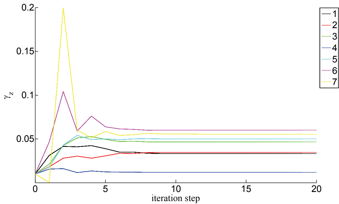
Fig. 7. Evolution of the damping parameters \gamma_z ( z=1,\dots,7 in the legend) during iterations by adopting the proposed updating procedure. Example with 12 measurement response dofs and without noise.
