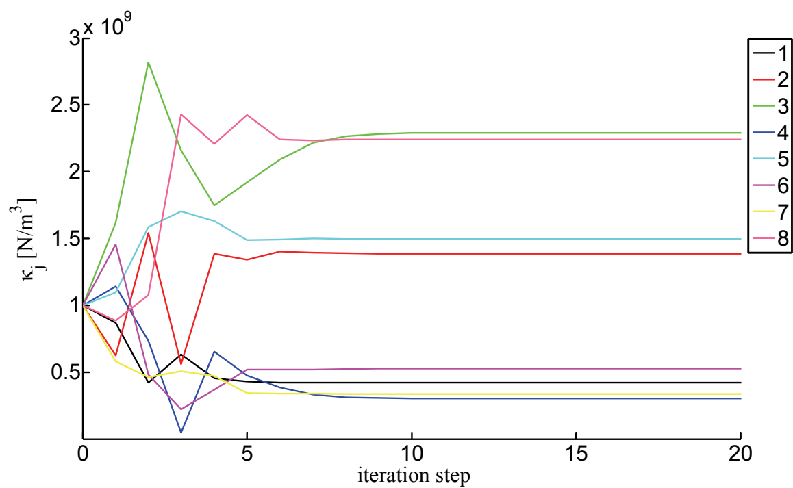
Fig. 14. Evolution of stiffness parameters \kappa_j ( j=1,...,8 in the legend) during iterations by adopting the proposed updating procedure. Example with 4 measurement response dofs and with 3% noise.
