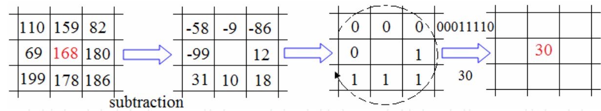
Fig. 6. An example of LBP calculation.
