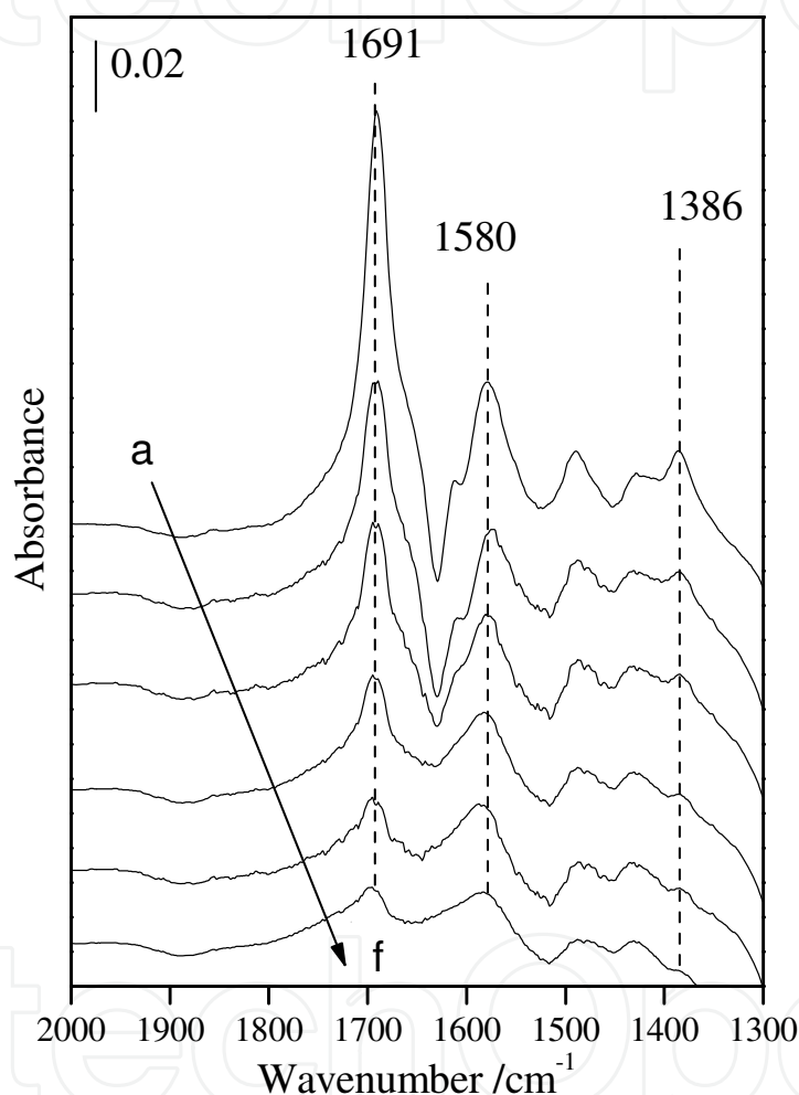
Fig. 31. FTIR spectra of surface species on 2%Zr/FER at 300 °C when the catalyst was exposed to 500 ppm \text{C}_2\text{H}_2 + 1000 ppm \text{NO} + 10 % \text{O}_2 + \text{N}_2 for 25 min (a) and subsequently exposed to 1000 ppm \text{NO} + 10 % \text{O}_2 + \text{N}_2 for 1 min (b), 5 min (c), 10 min (d), 15 min (e) and 30 min (f)
