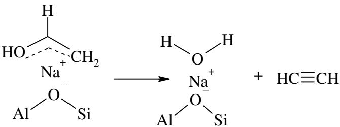
Scheme 3. The decomposition of carbonous species on NaZSM-5
