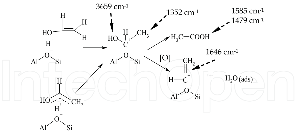
Scheme 2. The evolution of carbonous species on HZSM-5
