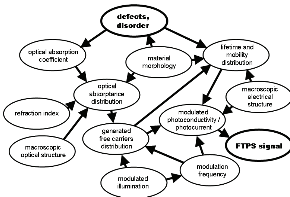
Fig. 6. Diagram shows most of the possible effects playing between defects density and disorder as input that we want to know and FTPS signal as output that we measure
