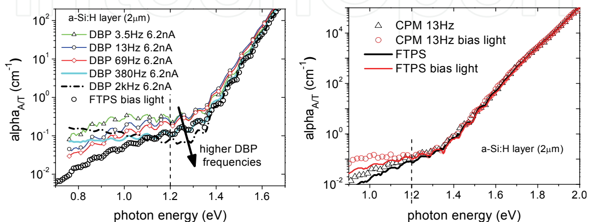
Fig. 8. Left: Dual Beam Photocurrent (DBP) spectra on 2μm amorphous Si on glass converge at higher frequencies to FTPS under bias light, at 380Hz and 2kHz DBP show anomalous deviation due to displacement currents. Right: Similar effect of light bias on FTPS and CPM methods and their comparison on the same sample
