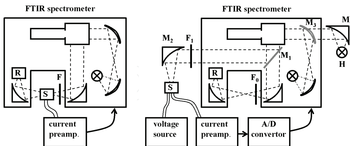
Fig. 3. On the left: 'simplest' FTPS setup where sample S is inside the sample area, reference R is measured without sample and with filter F (generally different for sample and reference). On the right: 'richest' FTPS setup with beam reflected out by sliding mirror M 1 to external focusing mirror M 2 , two different positions for filter F 0 , F 1 , external source H , external mirror M 4 , rotating mirror M 3 , external A/D convertor and voltage source
