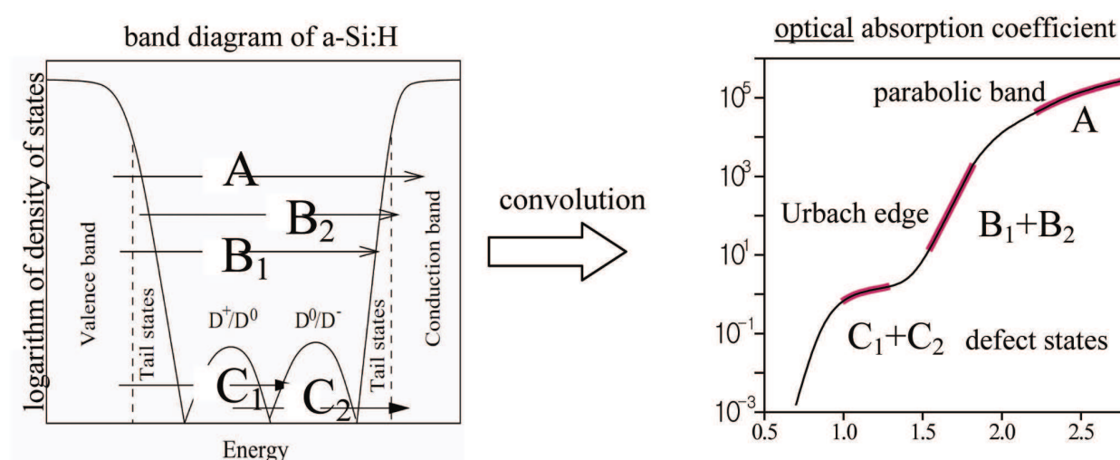
Fig. 1. On the left: band structure of density of electronic states of amorphous silicon On the right: optical absorption coefficient curve with indicated regions attributed to different electron transitions - desired result of photocurrent spectroscopy
