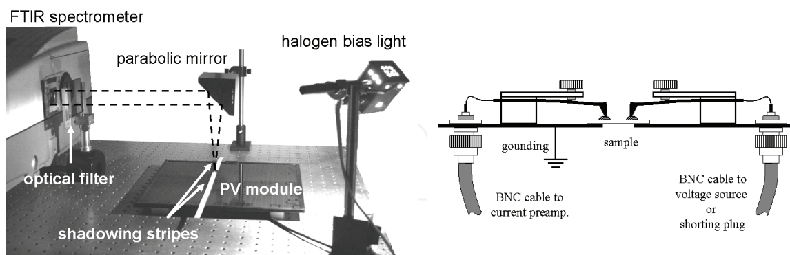
Fig. 4. On the left: FTPS setup with the use of external focusing mirror for measurement of maps of density of defects of PV modules. For selecting one spot shadowing stripes and bias light was used. On the right: sample holder for layers on glass and solar cells that have both contacts on the same side of glass substrate
