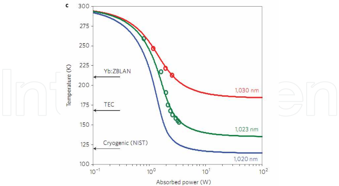
Fig. 2.12. Dependences of the sample cooling temperature on the absorbed power for different pump laser wavelength. The open circles are the experimental data and the solid lines are the mode fitting curves from Eq. 2.10. The blue line indicates the sample used in the experiment can achieve the minimum temperature. (Figure from ref. [23])
