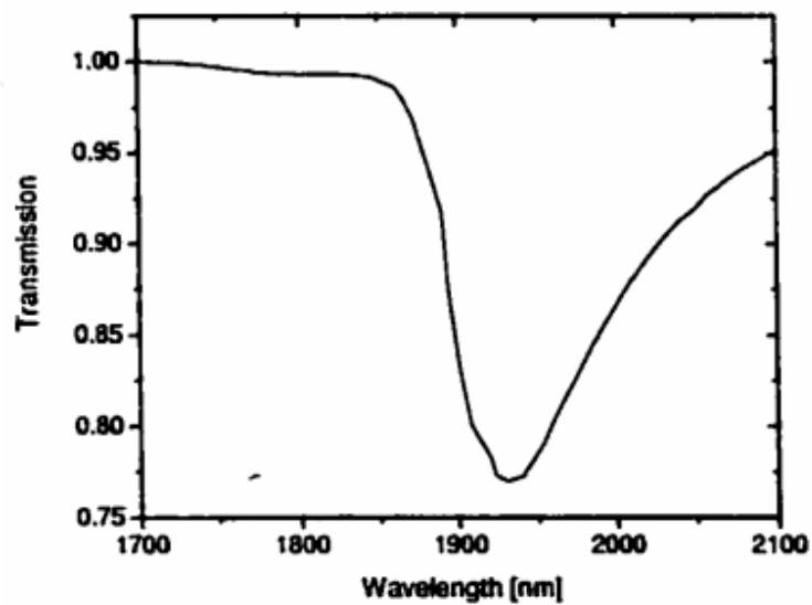
Fig. 2.6. Transmission spectrum of the cooling sample with a length of 20 μ m (figure from ref. [4])
