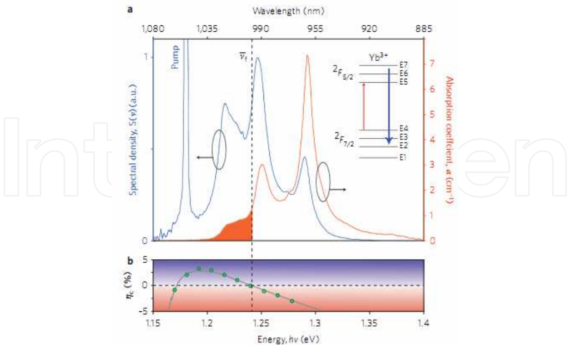
Fig. 2.11. Absorption, emission and cooling efficiency spectra of the 5% doped \text{Yb}^{3+} YLF crystal. The red and blue lines are the absorption and emission spectra respectively for a pump laser with \lambda=1055\text{nm} and polarization along the c-axis. The shade of the red line is the cooling tail. Inset: 2F_{5/2} and 2F_{7/2} levels in the crystal position containing seven stark manifolds. Figure b, cooling efficiency curve, the open circles is the experimental data and the line is the mode fitting one. (Figure from ref. [12])
