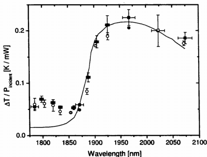
Fig. 2.5. Mirrored sample heating with qualitative fit using water absorption (figure from ref. [4])
