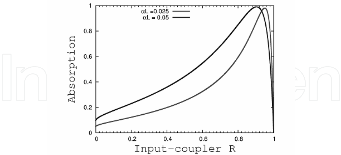
Fig. 4.4. The relationship between the cavity-enhanced absorption and the input-coupler reflectivity for two different values of \alpha l (Figure from ref. [13]) From the extra-cavity enhancement theory in section 3.1, D. Seletskiy calculated the input-coupler reflectivity as a function of the sample absorption for different optical density \alpha l , and the results are shown in Fig. 4.4. In the experiment, D. Seletskiy et al demonstrated the absorption enhancement for two different input-coupler reflectivities, and the results are shown in Fig. 4.5. We can see from the theoretical calculation (see Fig.4.4) and the experimental results (see Fig.4.5) that the experimental data are in good agreement with the theoretical results, which can be further found in Fig. 4.6. In this work, D. Seletskiy et.al did not give the temperature drop of the sample, but just to prove the enhancement of resonant absorption of Yb: ZBLAN glass sample by a factor of 11 compared to the double-pass configuration. This is the great significance meaningful work because it has relatively simple optical arrangement and great enhancement of the absorption for the cooling sample.
