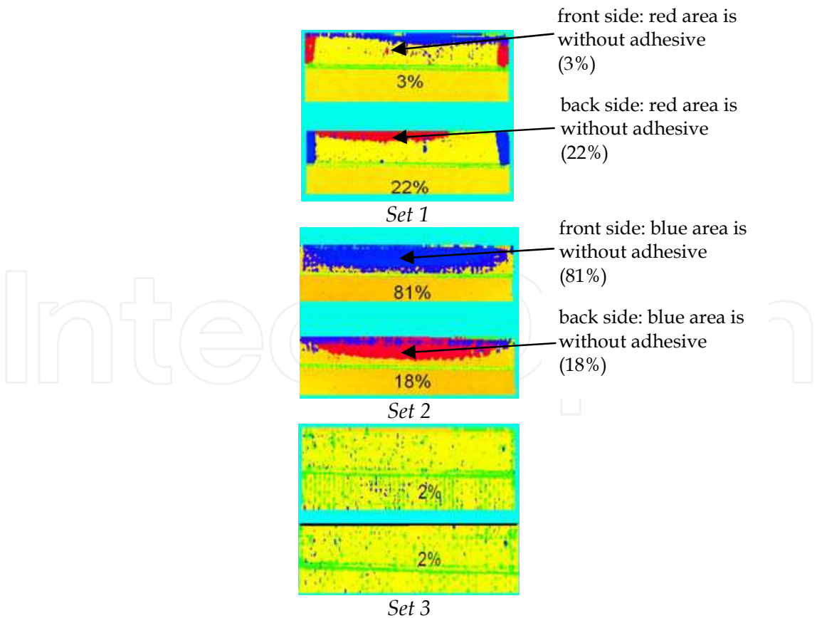
Fig. 17. C-scan images of the specimens indicating the amount of imperfect bonding.
