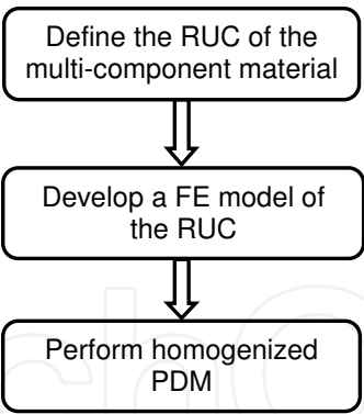
Fig. 8. Flowchart of the multi-scale damage model.
