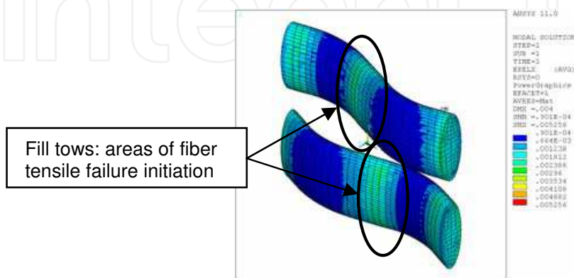
Fig. 13. Contour of longitudinal strain in fill tows and indication of fiber tensile failure initiation.
