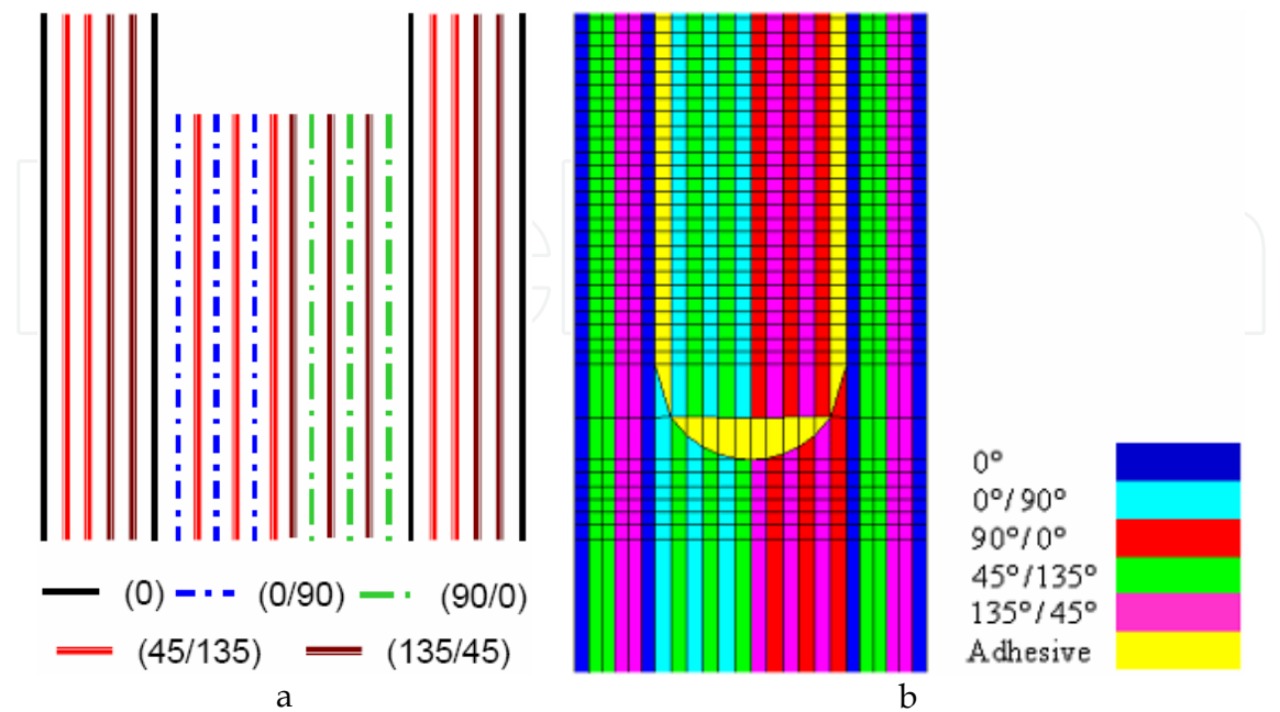
Fig. 16.a. Schematic description of the lay-up and b. Front-view of the FE mesh of the DLS joint.
