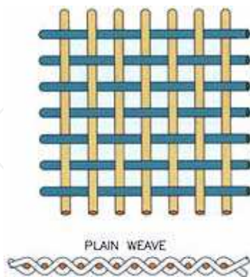
Fig. 7. Schematic of the plain weave composite material.
