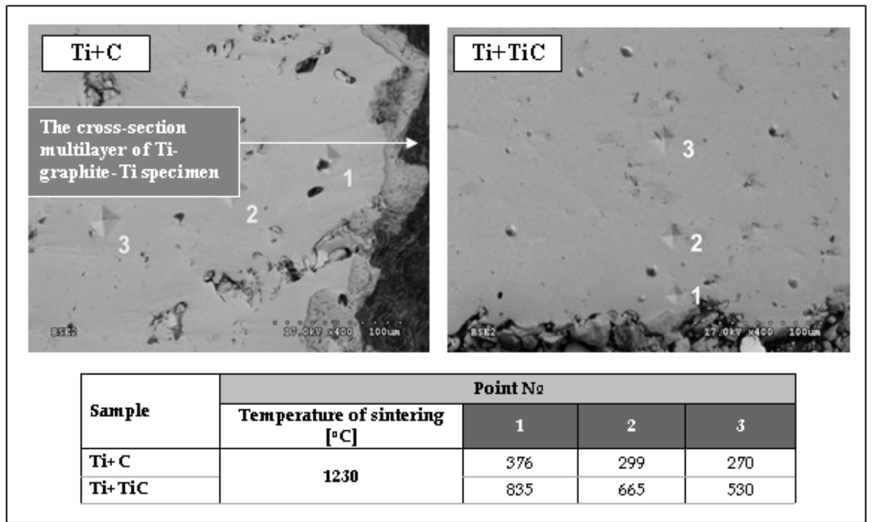
Fig. 9. Influence of carbon diffusion on microhardness of titanium samples A comparison of the friction coefficient values for the investigated materials is shown in Fig. 10. The analysis of the obtained results confirmed a good influence of graphite on tribological properties of the sinters. The friction coefficients for the composites with graphite reduced over twice compared with friction of pure titanium samples. The values of the motion resistance are also lower for the composites with titanium carbide, although to a lesser degree than in the case of the composites with graphite. In two cases, the influence of modifiers is clearly visible – an
