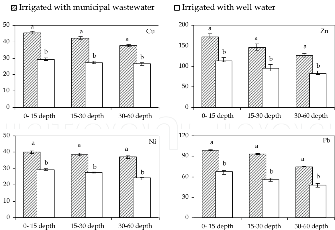
Fig. 1. Comparison of heavy metals in similar depths (0-15, 15-30 and 30-60 cm) between soils irrigated with wastewater and well water (mg/kg); Error bars are \pm SE
