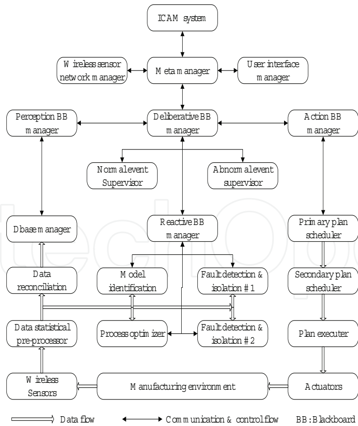
Fig. 4. ICAM system architecture and behavior model
