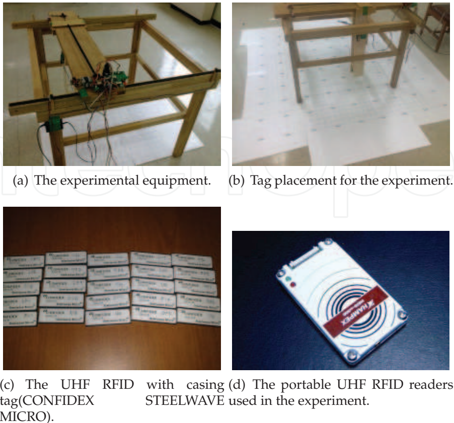
Fig. 6. The experimental settings.
