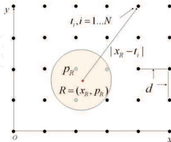
Fig. 1. Concept of the RFID tag floor localization method.
