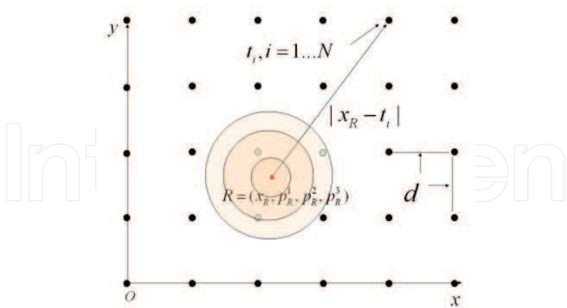
Fig. 2. The concept of the RFID tag floor localization method with multiple recognition ranges.
