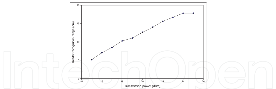
Fig. 8. Experimental result of the relation between reader transmission power and reader recognition range
