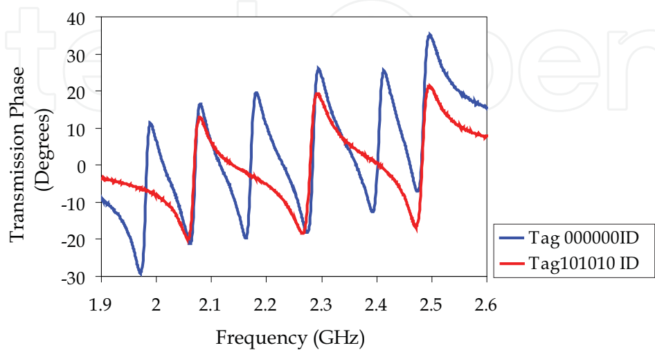
Fig. 20. Measured transmission phases of chipless tags with different spectral signatures.
