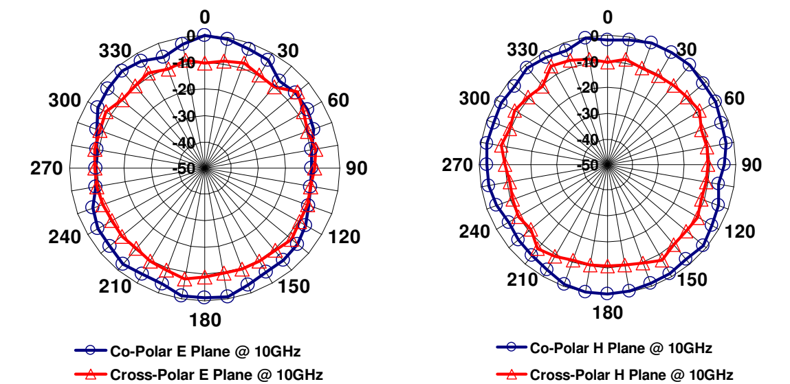
Fig. 26. Measured co-polar and cross-polar radiation patterns of UWB monopole at 10 GHz.
