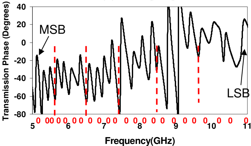
Fig. 29. Measured tag transmission phase of 23 bit tag ID "0x000000".
