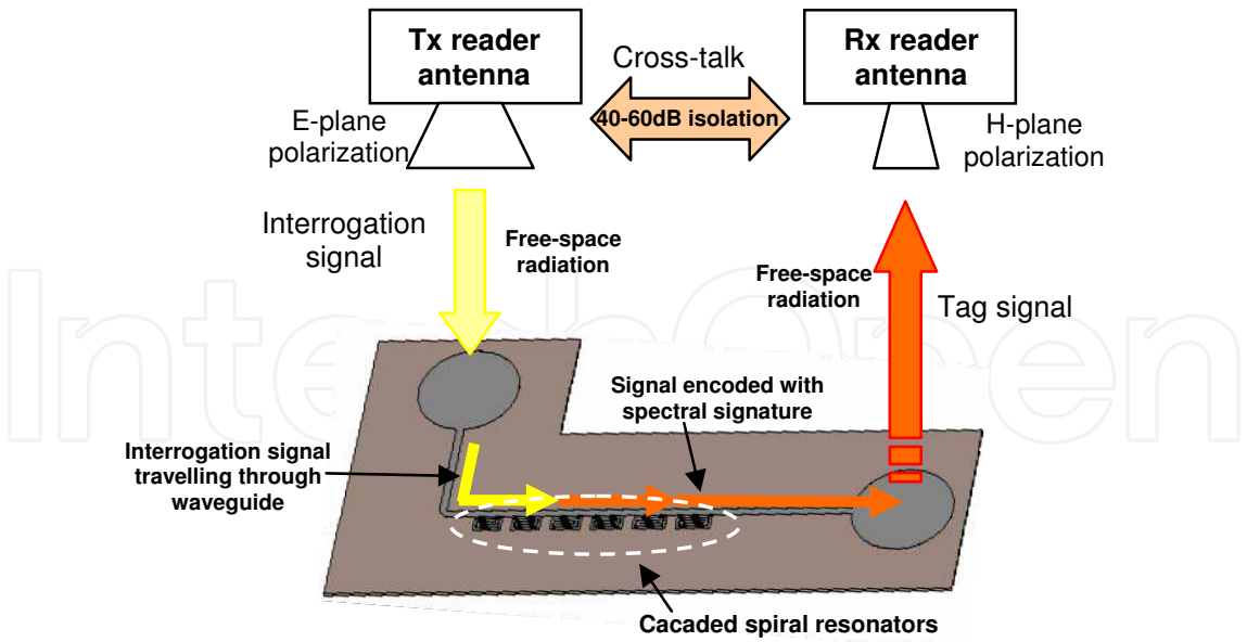
Fig. 7. Chipless RFID system signal flow diagram.
