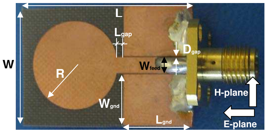
Fig. 11. Photograph of CPW fed UWB monopole ( L = 27\text{ mm} , W = 18.8\text{ mm} , L_{\text{gnd}} = 12\text{ mm} , W_{\text{gnd}} = 8\text{ mm} , D_{\text{gap}} = 0.15\text{ mm} , L_{\text{gap}} = 2\text{ mm} , W_{\text{feed}} = 2.5\text{ mm} and R = 7\text{ mm} , substrate Taconic TF-290 \epsilon_r = 2.9 , h = 0.09\text{ mm} , \tan\delta = 0.0028 ).
