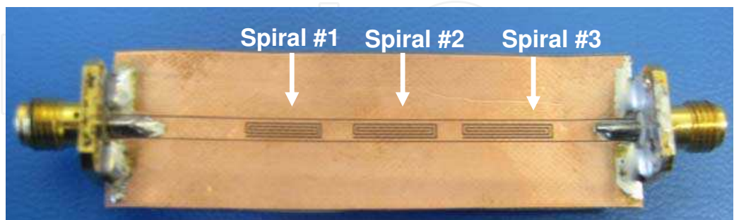
Fig. 15. Photograph of manufactured CPW 3-bit multiresonator on 90 \mu\text{m} Taconic TF-290 substrate.
