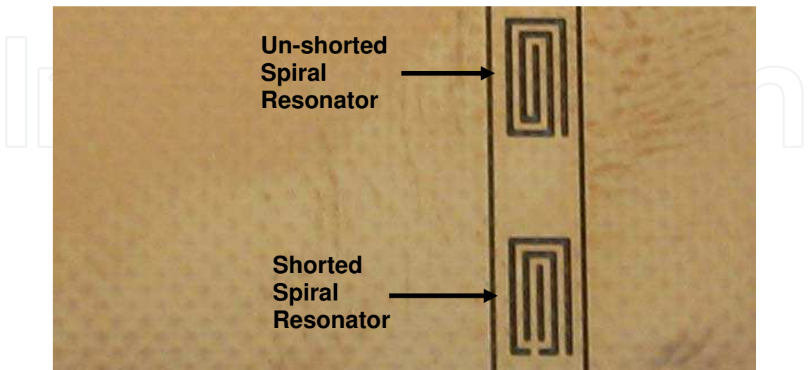
Fig. 17. Photograph of removing spiral resonances via spiral shorting for CPW multiresonator.
