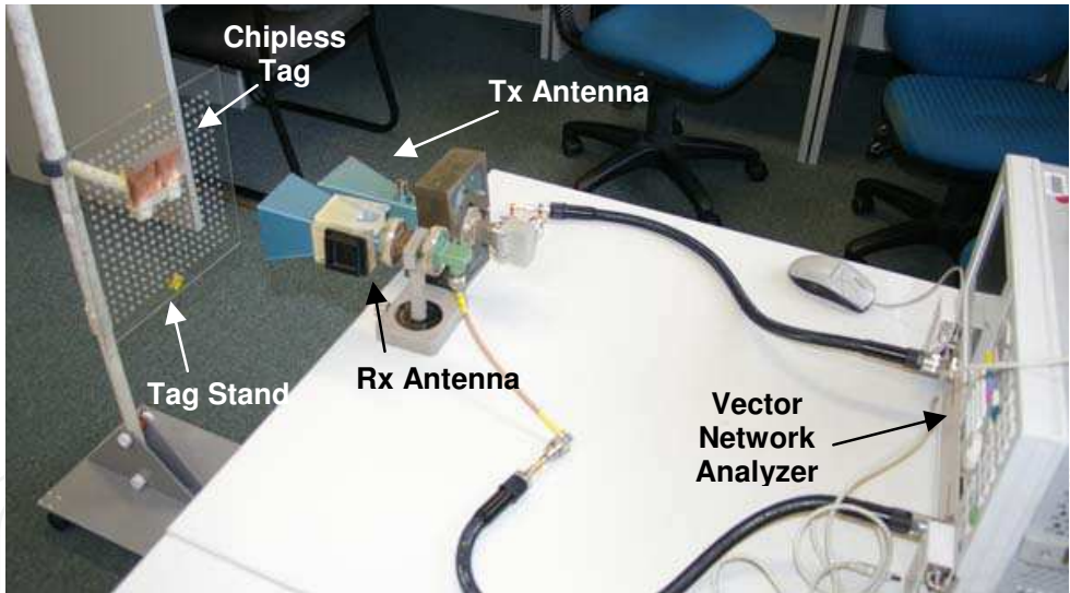
Fig. 37. Photograph of the experimental setup in the laboratory. Fig. 36 shows that the tag was read accurately in both amplitude and phase up to 15 cm when placed in a laboratory as shown in Fig. 37. The phase data were detectable at greater reading ranges (up to 35 cm) than the amplitude data due to robustness of the phase data. Fig 36 clearly shows that the reading range dropped by 50% outside the anechoic chamber due to interference from the environment. However, it should be mentioned that the detection procedure was a simple comparison of tag data with no resonances and tag data with all resonances. The reading range could be improved by using signal processing techniques (such as matched filtering) to isolate the tag signal from the noise and interference and thus increase the reading range (Hartmann et al, 2004).
