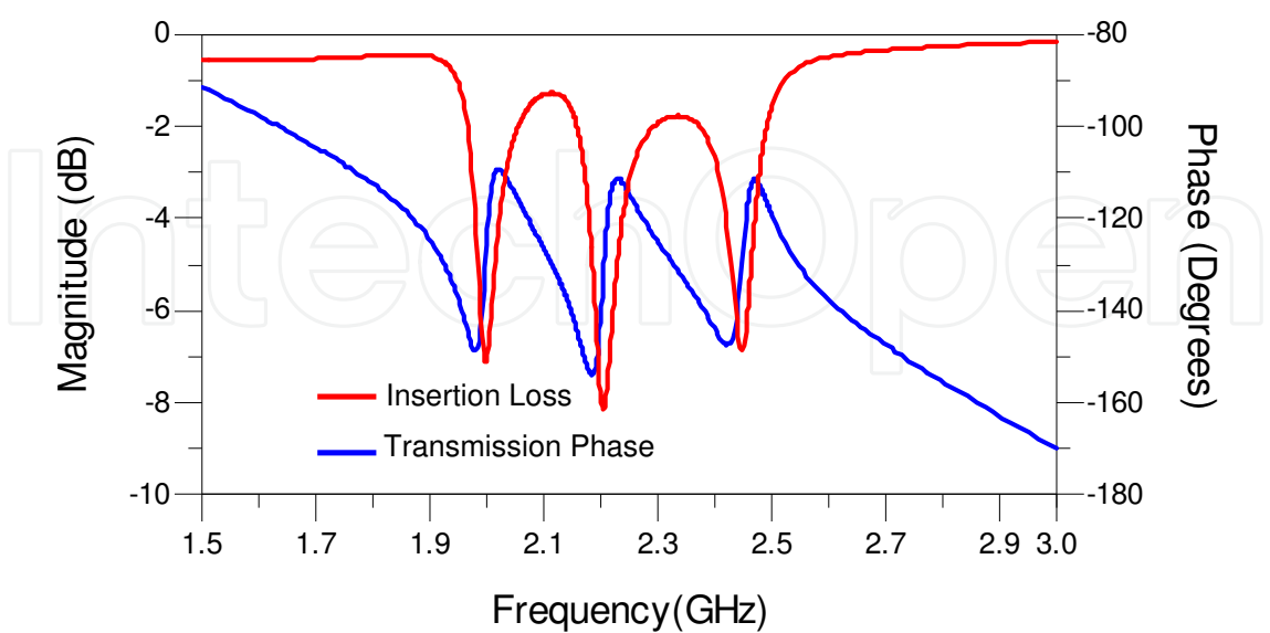
Fig. 16. Measured insertion loss and transmission phase of CPW 3-bit multiresonator.
