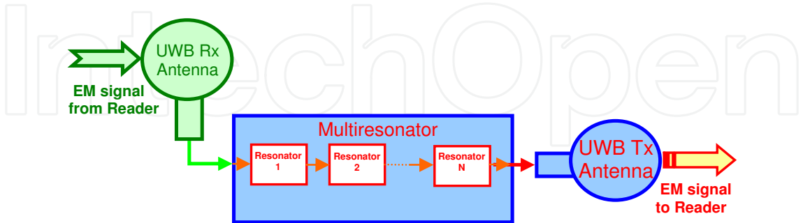
Fig. 5. Block diagram of chipless RFID tag.
