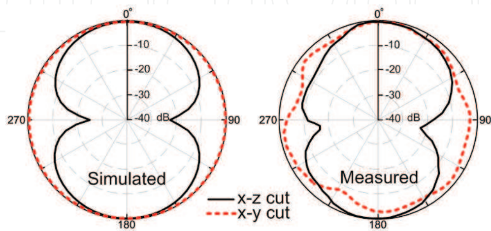
Fig. 11. Radiation patterns for 900 MHz
