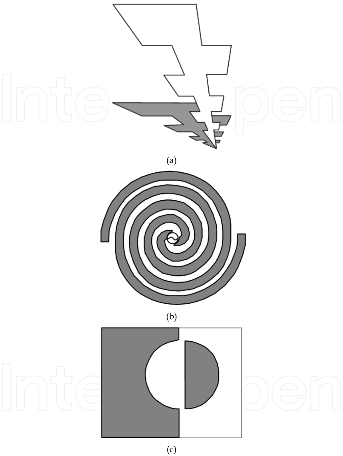
Fig. 4. Self-complementary antenna configurations, (a) log-period (b) spiral (c) circular disk A typical circular polarization dipole cross-pair usually consist of two individuals with horizontal and vertical locations, and a two-phase signal with 90° difference. Fig. 7 illustrates the simulated current distributions and Fig. 6 depicts the simulated electric fields among the planar structures, which provide a clearly physical insight on understanding the circular polarization of the proposed antenna. Fig. 5 shows that the Hilbert-curve is excited
