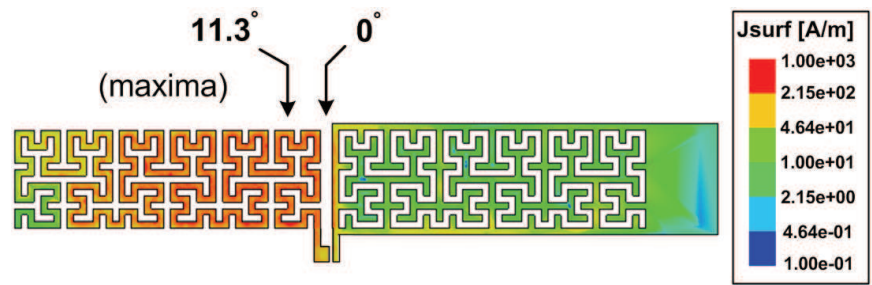
Fig. 7. Current distributions
