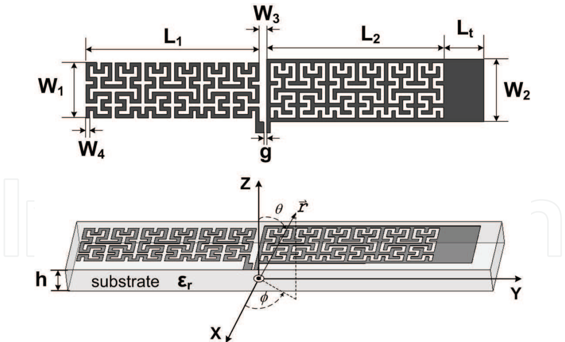
Fig. 6. Dimensions of complementary Hilbert-curve tag antenna
