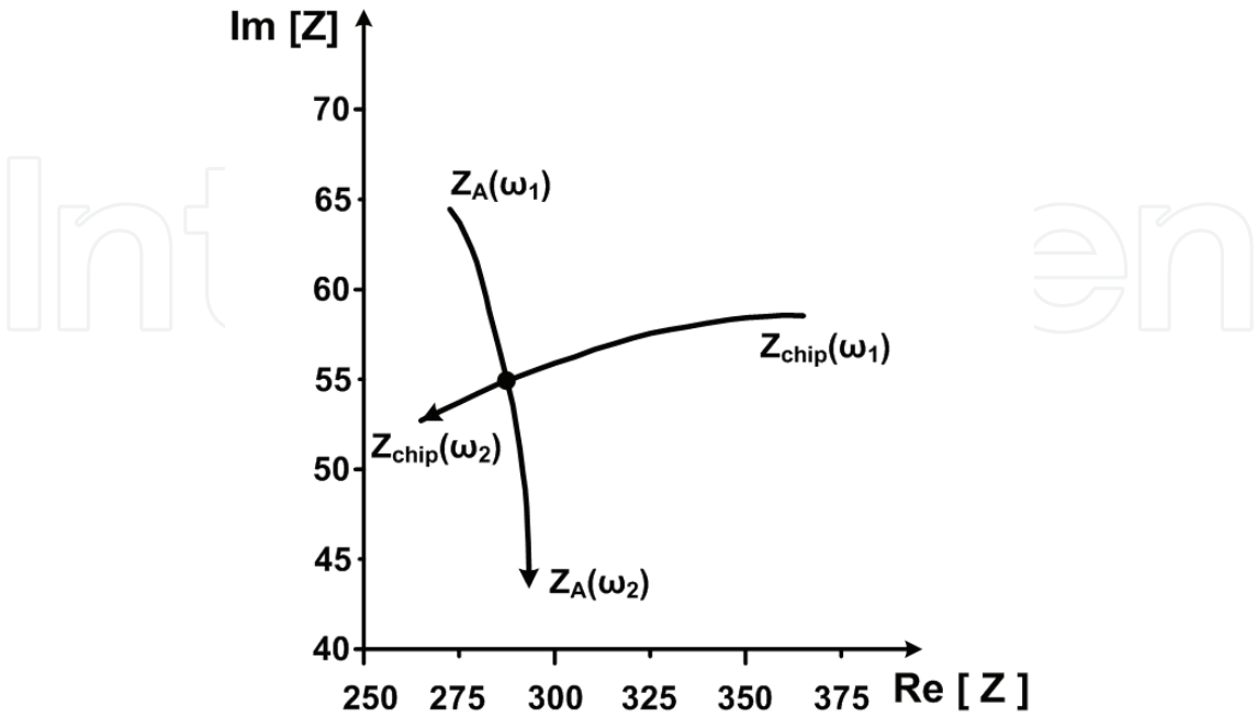
Fig. 13. Impedance locus
