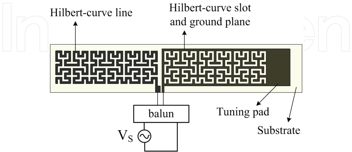
Fig. 5. Complementary Hilbert-curve antenna
