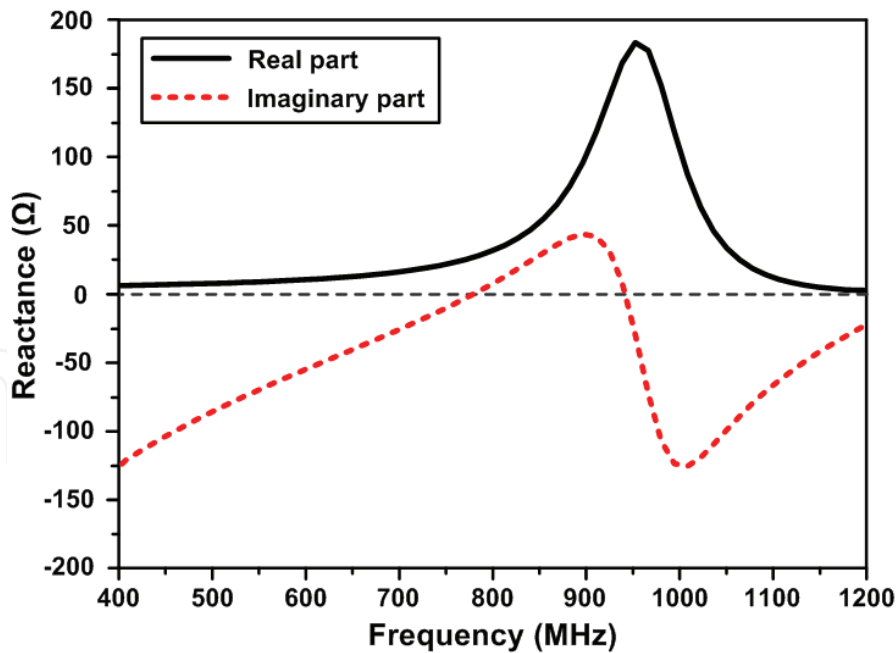
Fig. 10. Simulated results of impedance spectrum
