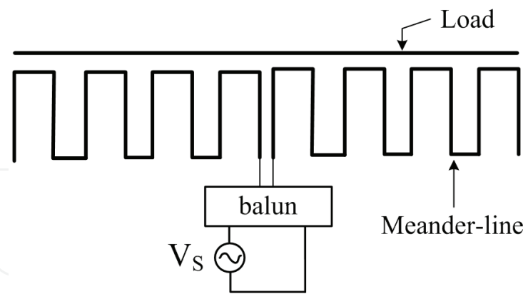
Fig. 2. Meander line antennas
