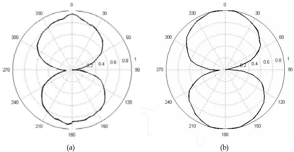
Fig. 19. Measured radiation pattern for the fabricated antennas, (a) (S3-45°) antenna and (b) (S3-60°) antenna. From Fig. 19, maximum measured gain of (0.948) dBi is obtained for (S3-45°). The measured radiation pattern was carried out for \varphi=0 . The Return Loss of the fabricated fractal dipoles is measured using (MOTTECH RF-2000) and plotted as shown in Fig. 20. From Fig. 20, a measured RL of (-27) dB could be compared with the simulated RL of (-15.12) dB given in Table 7 for (S3-45°) while measured RL of (-27) dB is compared with simulated RL of (-12.6) dB given in Table 7 for (S3-60°).
