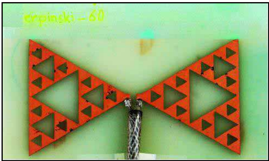
Fig. 17. The fabricated S3-60° antenna.
