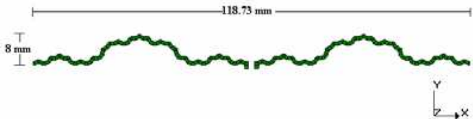
Fig. 6. The modified Koch fractal dipole antenna (K3-27.5°).
