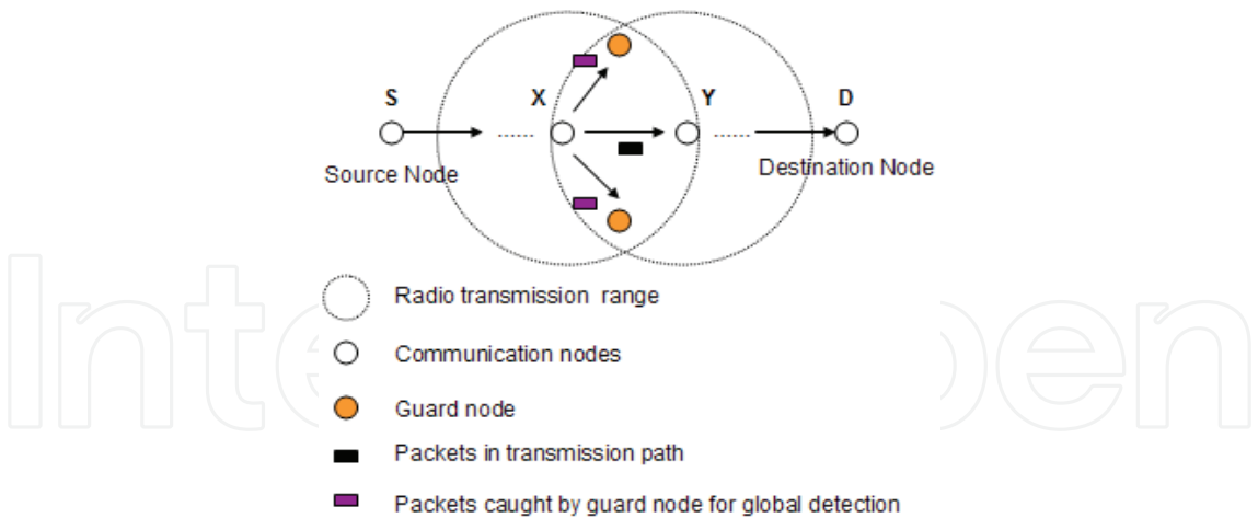
Fig. 2. Monitor node
