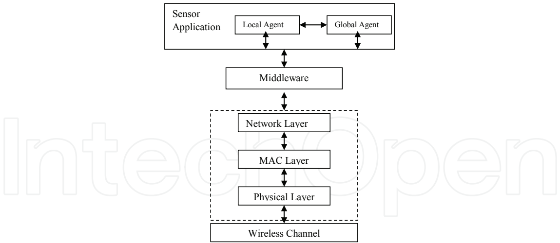
Fig. 1. Intrusion detection agents on sensor protocol’s stack
