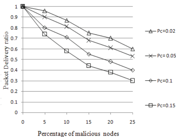
Fig. 14. Packet delivery ratio under attacks
