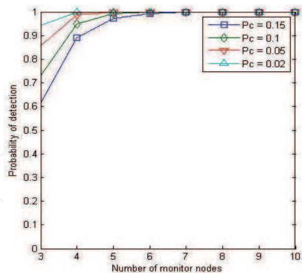
Fig. 12. Detection probability of a malicious node
