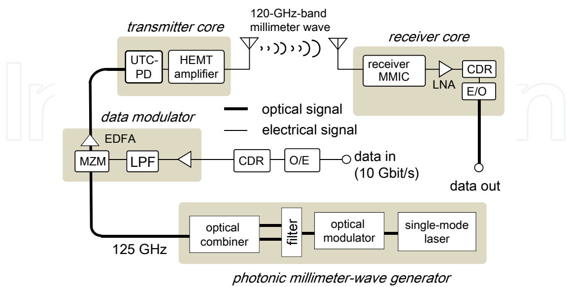
Fig. 15. Block diagram of 120-GHz band wireless link system using the UTC-PD in the transmitter.
