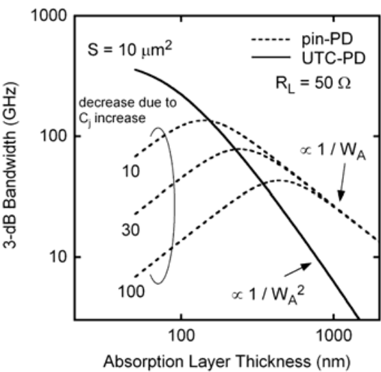
Fig. 4. Calculated relationships between f_{3dB} and W_A for UTC-PD and pin-PDs.
