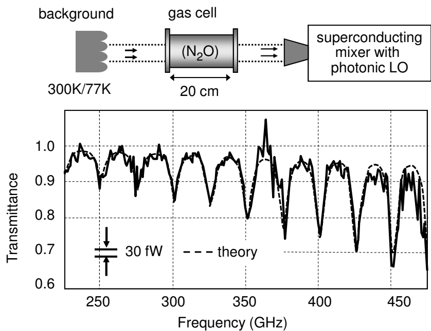
Fig. 20. Passive spectroscopic measurement of gas.
