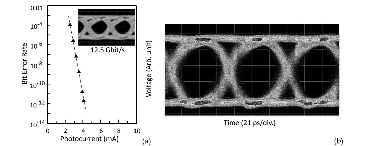
Fig. 17. (a) BER characteristics of 300-GHz wireless link. (b) 14-Gbit/s eye diagram. Figure 17(a) shows BER characteristics at 12.5 Gbit/s with a carrier frequency of 300 GHz. Horizontal axis is a photocurrent of the transmitter. An error-free transmission at 12.5 Gbit/s has been achieved with 4-mA current, which corresponds to the transmitter output of around 10 \mu W. Currently, the upper limits in the bit rate of PPG and BER tester are 14 Gbit/s and 12.5 Gbit/s, respectively. Figure 17(b) shows the eye diagram at 14 Gbit/s. Although the BER could not be measured, an error-free transmission was confirmed from the clear eye opening. Based on the design, >20Gbit/s will be feasible.
