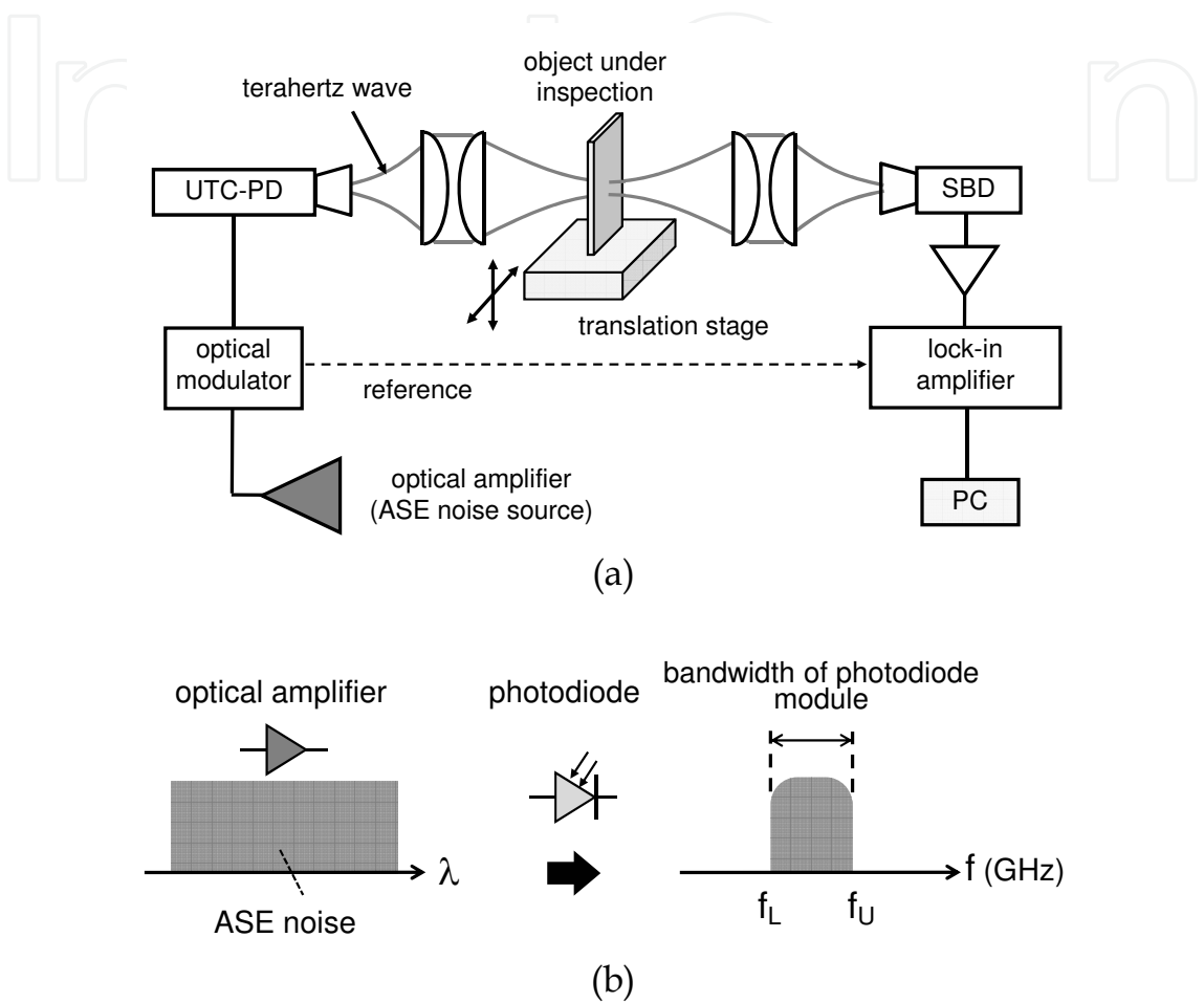
Fig. 23. (a) Block diagram of the imaging system using an incoherent noise source. (b) Mechanism of the noise generation using the photodiode.
