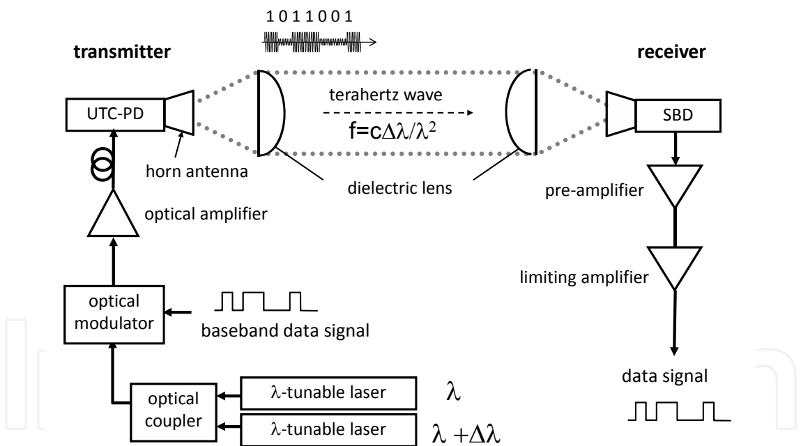
Fig. 16. Block diagram of 300-GHz band wireless link system using the UTC-PD in the transmitter.
