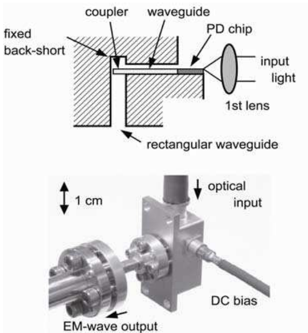
Fig. 7. Cross-sectional diagram and micrograph of a waveguide-output UTC-PD module. For the second approach, a quasi-optic UTC-PD module (Ito et al., 2005b) shown in Fig. 8 has been developed. Here, the UTC-PD was integrated with a planar antenna, and the device was mounted on a hyper-hemispherical lens made of high-resistivity silicon to collimate the output EM wave.
