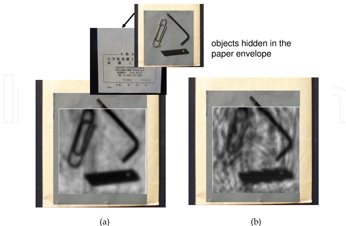
Fig. 24. Comparison of images obtained by noise source (a) and coherent source at 320 GHz (b).
