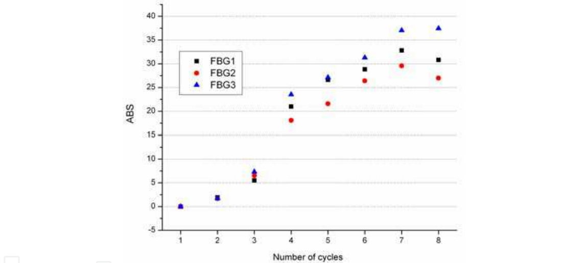
Fig. 12. Analysis of measurement results for final vessel loading cycles (detection of defects in structure of pressure vessel), (Gašior et al., 2007)
