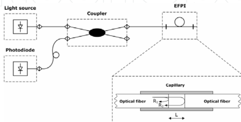
Fig. 3. Scheme of system based on extrinsic Fabry-Perot interferometric sensors
