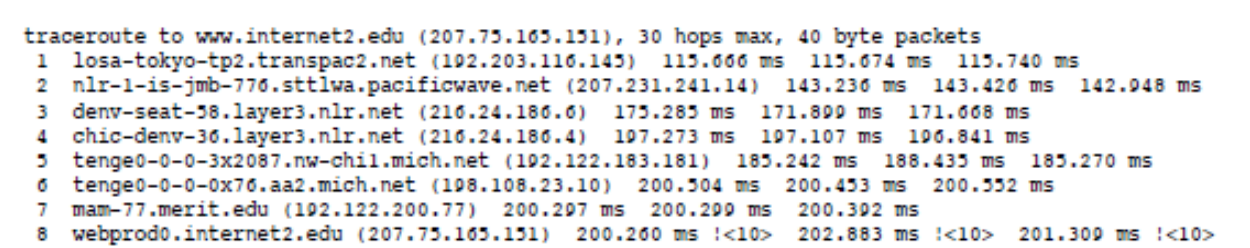
Fig. 12. Example of “traceroute” from APAN Tokyo XP to www.internet2.edu
