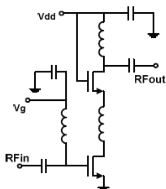
Fig. 8. The single-stage cascode LNA (Tao et al., 2009)
