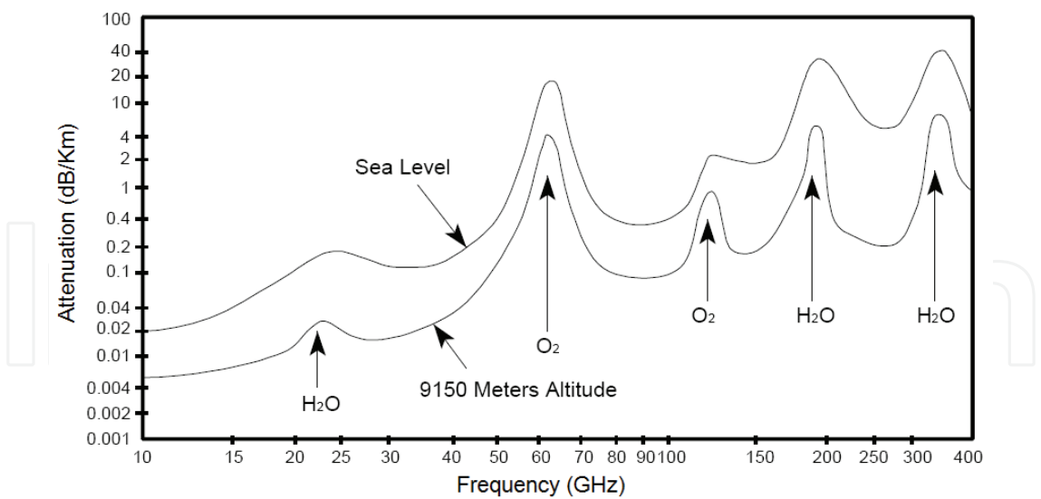
Fig. 1. The oxygen attenuation versus frequency (FCC, 1997)
