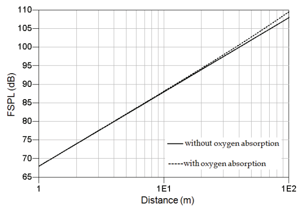
Fig. 2. The FSPL versus distance at 60 GHz
