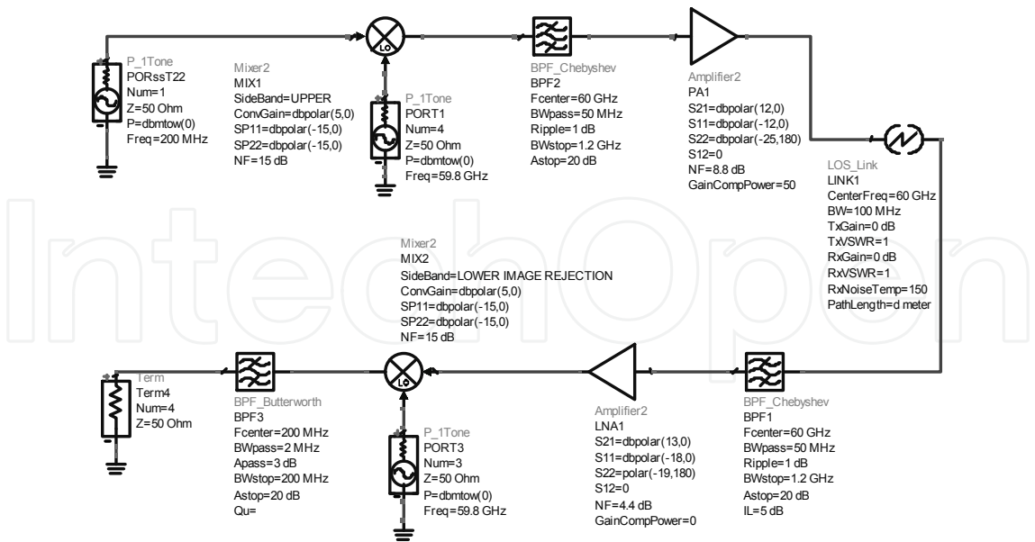
Fig. 5. The simulation setup with the characteristics of different building blocks
