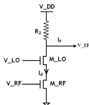
Fig. 9. The architecture of the dual-gate MOSFET mixer
