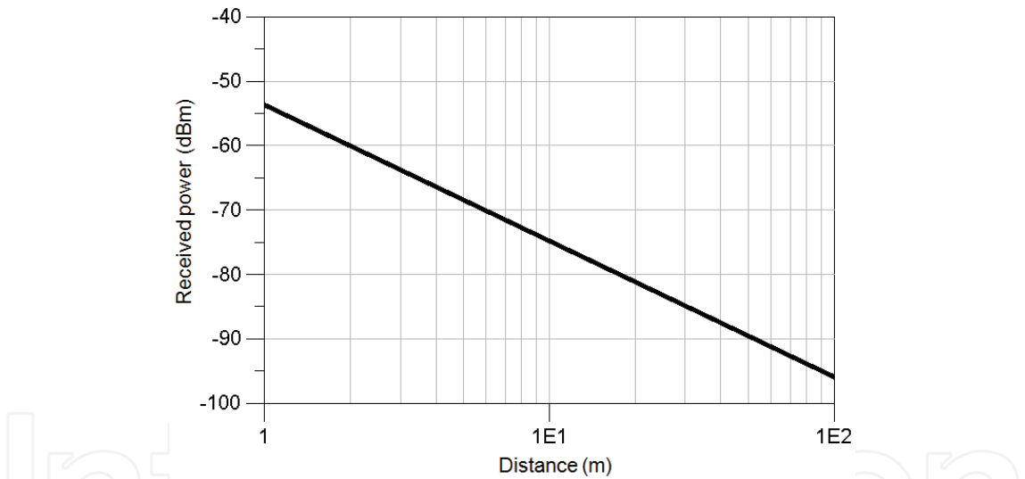
Fig. 6. The received power after demodulation at 60 GHz for a transmit power of 0 dBm vs. distance
