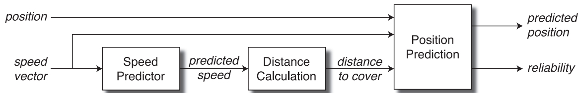
Fig. 1. Algorithm Outline
