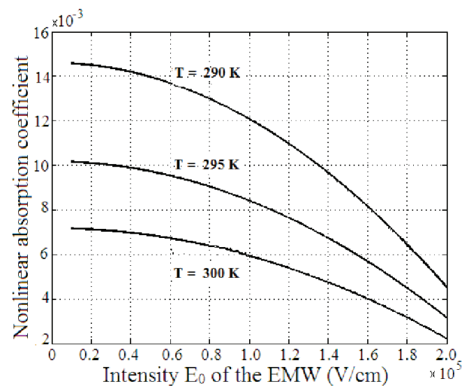
Fig. 4. The dependence of \alpha on E_0 in a quantum well
