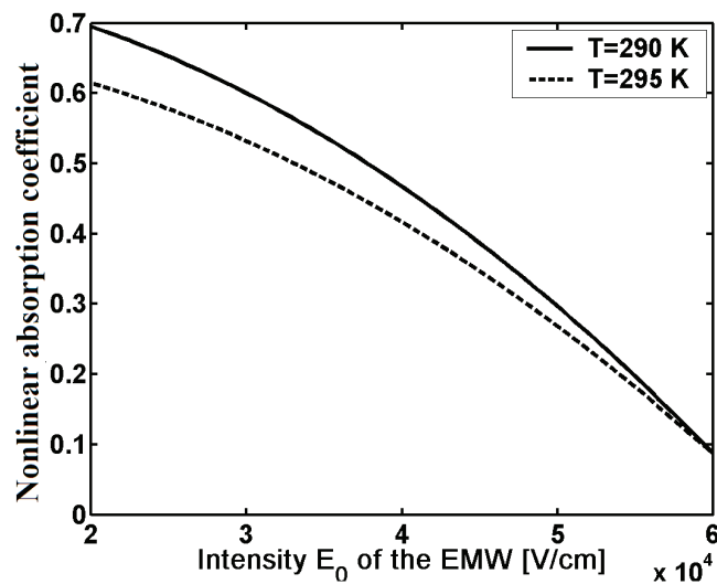
Fig. 12. The ependence of \alpha on E_0 in a cylindrical quantum wire (electron-acoustic phonon scattering)
